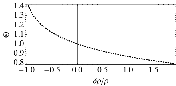
Figure 1. Function \Theta which corrects the relation of Eq. (1) when the density contrast is not linear. The plot assumes the Planck+BAO best-fit value of \Omega_m = 0.3086 , but the dependence of \Theta on cosmological parameters is very weak.
