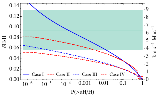
Figure 4. Probability of having an inhomogeneity that induces a \delta H/H (left vertical axis) or \delta H (right vertical axis) larger than a given value for the cases listed in the legend and in Table I. Also shown is the 1- \sigma band relative to the value H_{0,\text{unc}}^{\text{local}}/H_0^{\text{CMB}} - 1 .
