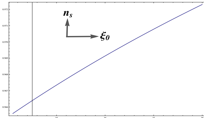
Figure 2: n_s vs \xi_0
