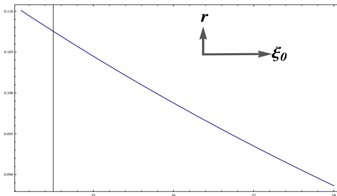
Figure 3: r vs \xi_0
