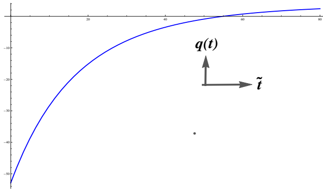
Figure 5: q(t) vs \tilde{t}
