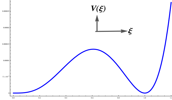
Figure 1: V(\xi) vs \xi
