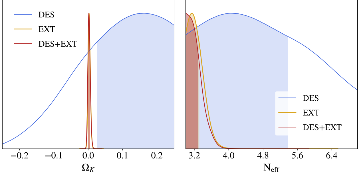
FIG. 2. Posterior constraints on the spatial curvature (left panel) and the number of relativistic species (right panel) in two of the extensions to \Lambda CDM considered in this paper. Blue contours show DES alone, yellow is external data alone, and red is the combination of the two. The 68% confidence region is shaded. Posteriors' maxima are normalized to unity for better visibility of the DES only results.
