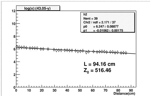
Fig. 3. Attenuation length for a typical scintillator strip
