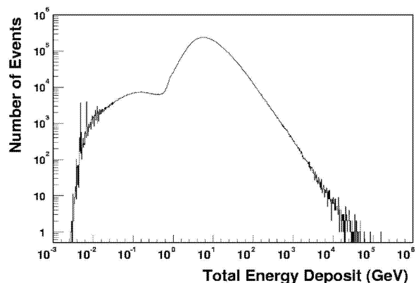
Fig. 5. All-particle spectrum in deposited energy.
