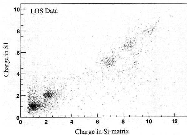
Fig. 6. Charge from Si-matrix versus charge from Scintillator S1.
