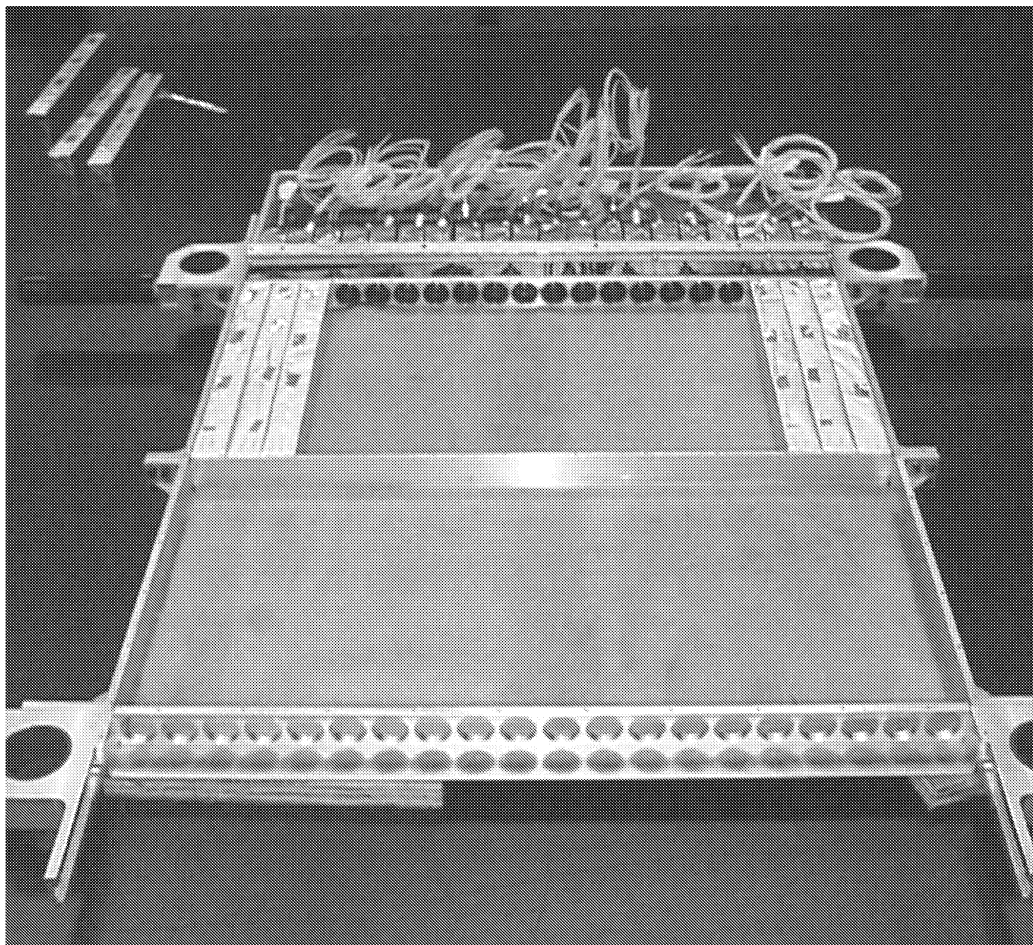
Figure 1. BGO tray top view
