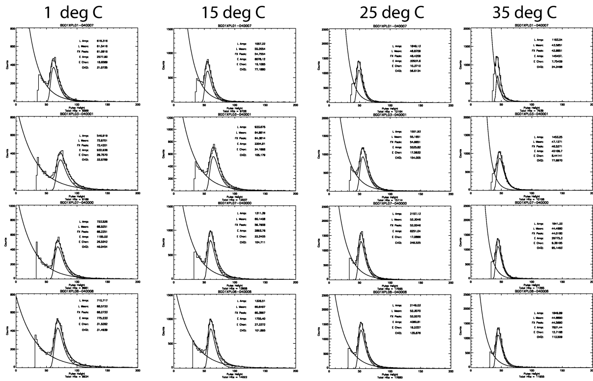
Figure 3. Muon peak histograms for 4 individual BGO crystals
