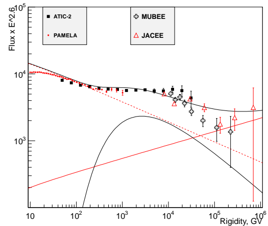
Figure 2. Proton energy spectrum as measured in the direct experiments and its fit to the model of local instantaneous source. Experimental data: PAMELA [18], ATIC-2 [17], MUBEE [19], JACEE [20]. Red dashed and solid lines are for background spectra, black lines – spectrum of single source and summary spectrum
