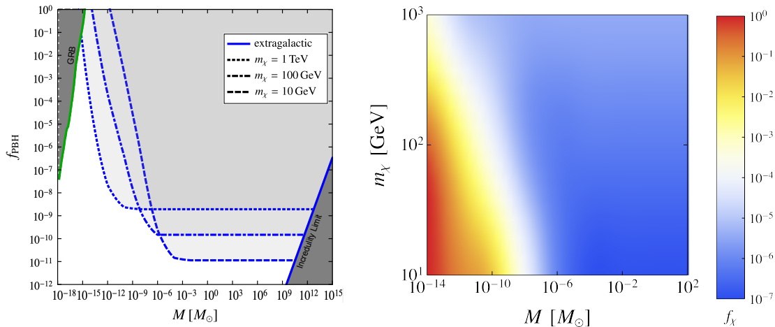
Figure 15: Constraints on f_{\text{PBH}} as a function of PBH mass (left) from extragalactic \gamma -ray background. Results are shown for m_{\chi} = 10 GeV (dashed lines), m_{\chi} = 100 GeV (dot-dashed lines) and m_{\chi} = 1 TeV (dotted lines), setting \langle\sigma v\rangle = 3 \times 10^{-26} \text{ cm}^3/\text{s} . Also shown is the extragalactic incredibility limit. The density plot (right) shows the fraction of WIMPs f_{\chi} (colour bar) as a function of the PBH mass M and of the WIMP mass m_{\chi} . We fixed f_{\text{PBH}} + f_{\chi} = 1 . Figures from Reference [229].
