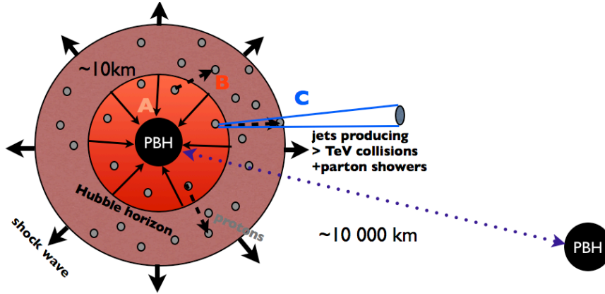
Figure 13: Qualitative representation of the three steps in the discussed scenario, from Reference [181]. (A) Gravitational collapse to a PBH of the curvature fluctuation at horizon re-entry. (B) Sphaleron transition in hot spot around the PBH, producing \eta \sim \mathcal{O}(1) locally through electroweak baryogenesis. (C) Propagation of baryons to rest of Universe through jets, resulting in the observed BAU with \eta \sim 10^{-9} .
