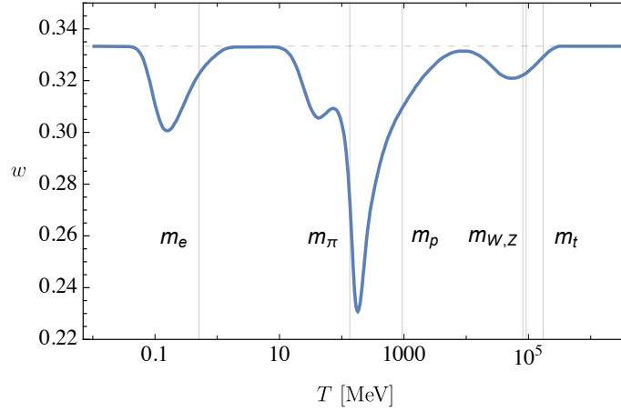
Figure 10: Equation-of-state parameter w as a function of temperature T , from Reference [32]. The grey vertical lines correspond to the masses of the electron, pion, proton/neutron, W/Z bosons and top quark. The grey dashed horizontal lines correspond to g_* = 100 and w = 1/3 .
