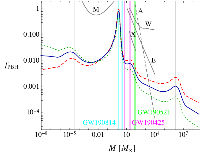
Figure 11: The mass spectrum of PBHs with spectral index n_s = 0.965 (red, dashed), 0.97 (blue, solid), 0.975 (green, dotted), from Reference [32]. The grey vertical lines corresponds to the electroweak and QCD phase transitions and e^+e^- annihilation. Also shown are the constraints associated with microlensing (M), wide-binaries (W), accretion (A), Eridanus (E) and X-ray observations (X). The vertical lines correspond to the gravitational-wave events GW190425 [182], GW190814 [183] and GW190521 [184, 185].
