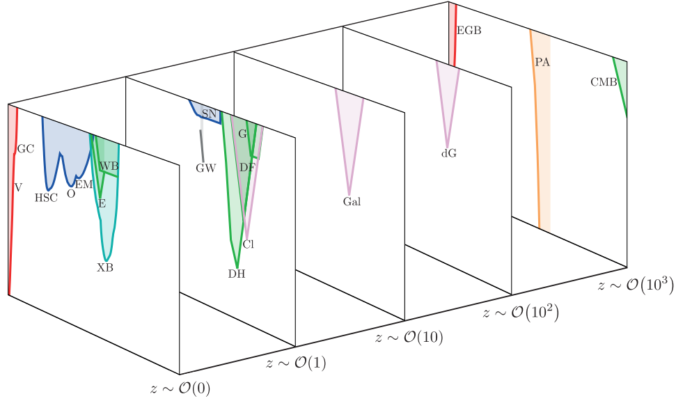
Figure 5: Limits shown in Figure 4 for different redshifts, from Reference [1]. The large-scale structure limit is broken down into its individual components from clusters (CI), Milky Way galaxies (Gal) and dwarf galaxies (dG), as these originate from different redshifts. Further abbreviations are defined in the caption of Figure 4.
