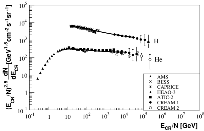
Figure 2. Fit to proton and He data with the spectral shape given in Stanev et al. (1993). For He, we use for the break energy 10 TeV/N, and for H 20 TeV, since the rigidity E/Z is given. For H, the strongest component is from ISM-SN, a wind component is required to fit the data, but is weaker. Replotting these spectra in energy per particle would shift He up by a factor of 8 and to the right by a factor of 4, at 10 TeV/N, and so give the crossover near that energy with H.
