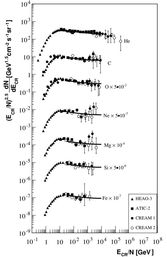
Figure 1. Fit for elements heavier than H with the spectral shape from Stanev et al. (1993). We use for the break energy 10 TeV/N and only fit the fluxes above 50 GeV/N because of solar modulation and low-energy spallation effects. No ISM-SN CR component is necessary to fit the spectra. Lower energy data imply a small ISM-SN CR component for He.
