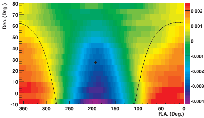
Figure 7. Result of a harmonic fit to the fractional difference of the CR rates from isotropic coordinates as viewed by Milagro for the years 2000–2007. The color bin width is 1.0 \times 10^{-4} reflecting the average statistical error. The two black lines show the position of the Galactic equator and the solid circle shows the position of the Galactic north pole. This map is constructed by combining 18 individual profiles of the anisotropy projection in R.A. of width 5^\circ in decl. It is not a two-dimensional map of the sky. The median energy of the events in this map is 6 TeV.
