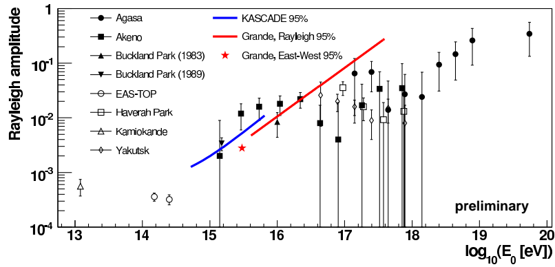
Figure 3: Upper limits for the Rayleigh amplitude, as obtained by a harmonic analyses of the distribution of the right ascension of arrival directions, compared to the results of other experiments.
