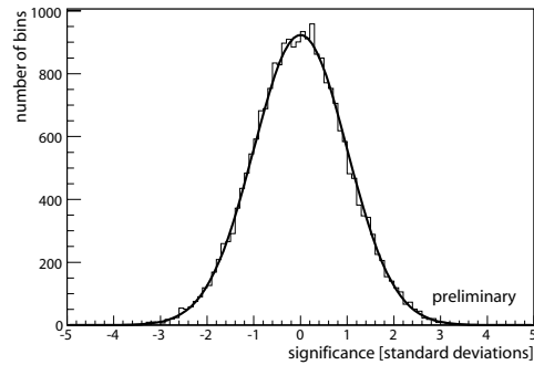
Figure 2: Distribution of the significance values of the 23216 bins containing events of the sky map. The plotted function depicts the expected behaviour: a gaussian function centered at 0 with a sigma of 1.
