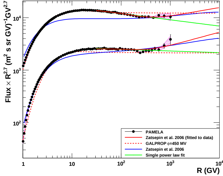
Figure 2: Proton (top points) and helium (bottom points) data measured by PAMELA in the rigidity range 1 GV - 1.2 TV. The shaded area represents the estimated systematic uncertainty. The lines represent the fit with a single power law and the Galprop (25) and Zatsepin (26) models. Details of the models are presented in Tables S1, S2.
