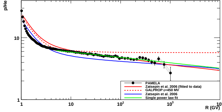
Figure 3: Ratio of the flux between proton and helium data of PAMELA vs. Rigidity. The shaded area represents the estimated systematic uncertainty. Lines show the fit using one single power law (describing the difference of the two spectral indices), the Galprop (25) and Zatsepin models with the original values of the paper (26) and fitted to the data. Details of the models are presented in Tables S1, S2.
