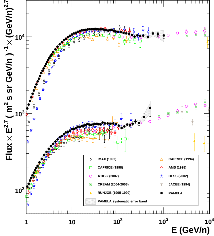
Figure 1: Proton and helium absolute fluxes measured by PAMELA above 1 GeV/n, compared with a few of the previous measurements (14–22). All previous measurements but one (17) come from balloon-borne experiments. Previous data up to few hundred GeV/n were collected by magnetic spectrometer experiments (14–17, 19) while higher energy data come from calorimetric measurements. PAMELA data cover the energy range 1 GeV -1.2 TeV (1-600 GeV/n for He). The fluxes are expressed in terms of kinetic energy per nucleon, converted from the rigidity measured in the tracker and neglecting any contribution from less abundant deuterium ( d/p \simeq 1\% ) and ^3\text{He} ( ^3\text{He}/^4\text{He} \simeq 10\% ). Pure proton and ^4\text{He} samples are therefore assumed. Error bars are statistical, the shaded area represents the estimated systematic uncertainty.
