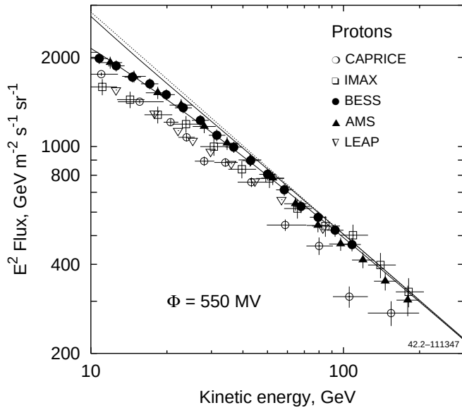
FIG. 2.—Proton spectrum as calculated in DR I/II models, compared with the data. Upper curve: LIS; lower curve: modulated to 550 MV. The dotted line shows the LIS spectrum best fitted to the data above 20 GeV (Moskalenko et al. 2002). Data: IMAX (Menn et al. 2000), CAPRICE (Boezio et al. 1999), BESS (Sanuki et al. 2000), AMS (Alcaraz et al. 2000), and LEAP (Seo et al. 1991).
