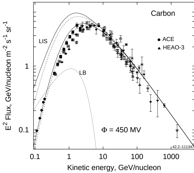
FIG. 4.—Spectrum of carbon calculated with (solid curves; DR II model) and without (dashed curves) LB contribution. Upper curves: LIS; lower curves: modulated using force field approximation ( \Phi = 450 MV). LB interstellar spectrum is shown as a dotted curve. Data: ACE (Davis et al. 2000, 2001) and HEAO 3 (Engelmann et al. 1990). For other references see Stephens & Streitmatter (1998) (symbols are changed).
