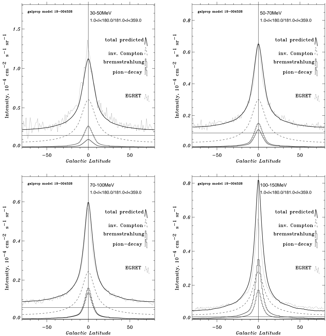
FIG. 14.—Latitude distribution of \gamma -rays ( 0^\circ \leq l \leq 360^\circ ) for model HEMN (thick solid line). Separate components show the contribution of IC (dashed line), bremsstrahlung (thin histogram), \pi^0 -decay (thick histogram); horizontal line, isotropic background; dotted line, EGRET data.
