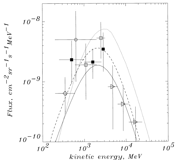
FIG. 9.—Interstellar antiproton flux for models (MSR98) compared with local measurements: solid line, C; dotted line, HN; dashed line, HEMN. Data (direct measurements): triangles, HEAT experiment (Basini et al. 1999); other points, see references in MSR98.
