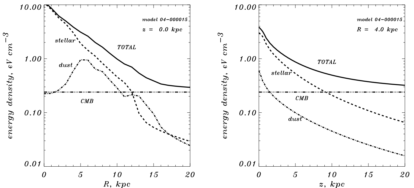
FIG. 1.—ISRF energy density as function of R at z = 0 (left), and of z at R = 4 kpc (right). Shown are the contributions of stars (dashed line), dust (dash-dotted line), CMB (dash-three-dotted line), and total (solid line).
