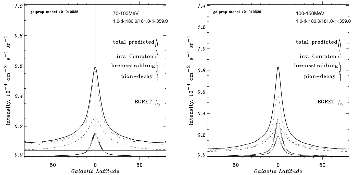
FIG. 19.—High-latitude distribution of \gamma -rays for HELH model, 70–100 MeV (left), and 100–150 MeV (right), compared to EGRET data. Lines are coded as in Fig. 14.
