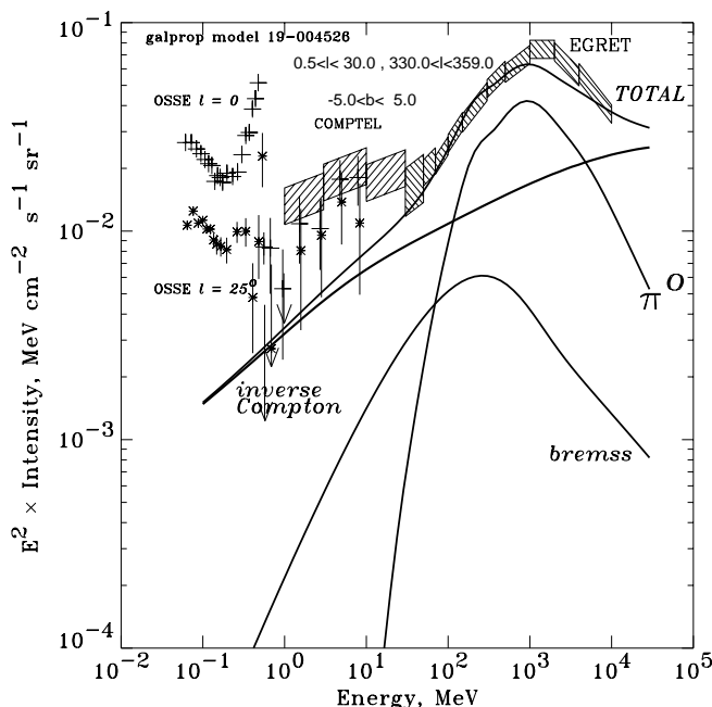
FIG. 13.—Gamma-ray data as in Fig. 7 compared with HEMN model (electron injection index = 1.8, and modified nucleon spectrum).
