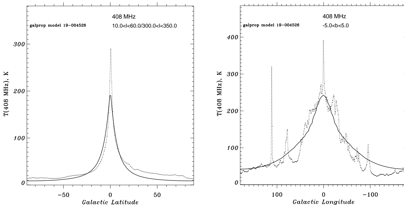
FIG. 5.—Intensity profiles of synchrotron emission at 408 MHz in latitude ( 10^\circ \leq l \leq 60^\circ , 300^\circ \leq l \leq 350^\circ ) and longitude ( |b| \leq 5^\circ ) for the HEMN model. Data: Haslam et al. (1982).
