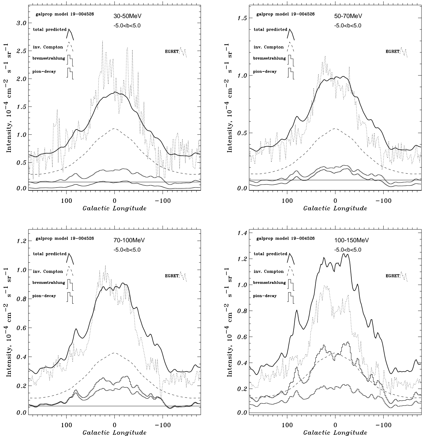
FIG. 15.—Longitude distribution of \gamma -rays ( |b| \leq 5^\circ ) for model HEMN. Coding of lines for components is the same as in Fig. 14. Dotted line: EGRET data.
