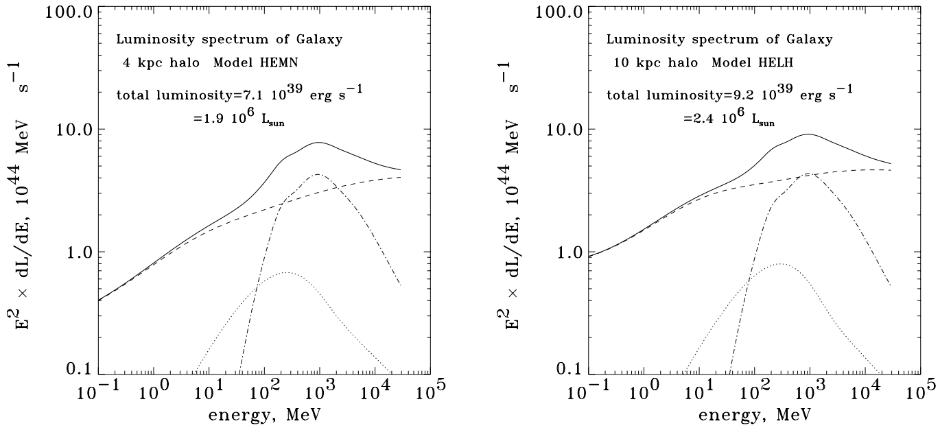
FIG. 20.—Gamma-ray luminosity spectrum of diffuse emission from the whole Galaxy using HEMN model ( left ), and HELH model ( right ). Total is shown as solid line. Separate components: IC ( dashed line ), bremsstrahlung ( dotted line ), and \pi^0 -decay ( dash-dotted line ).
