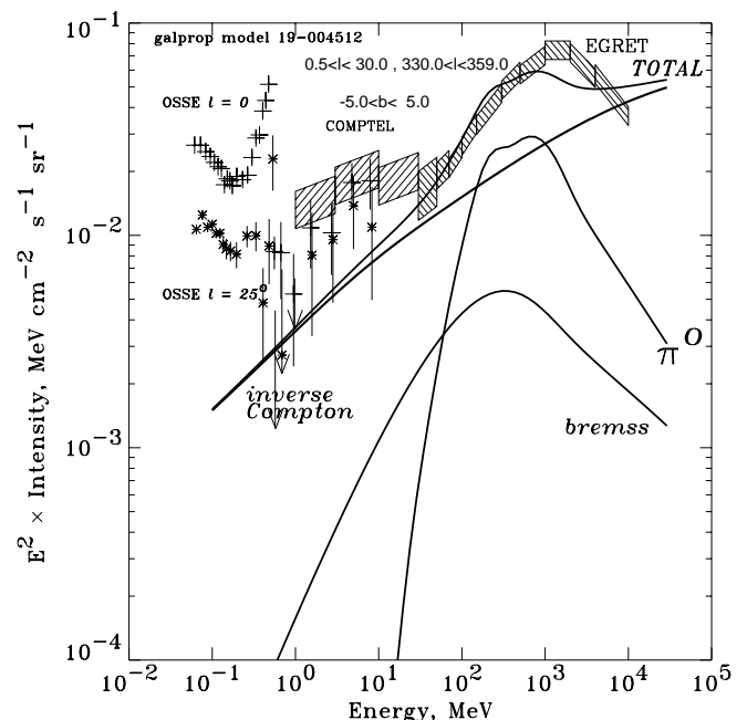
FIG. 12.—Gamma-ray data as in Fig. 7 compared with HE model (electron injection index -1.7 ).
