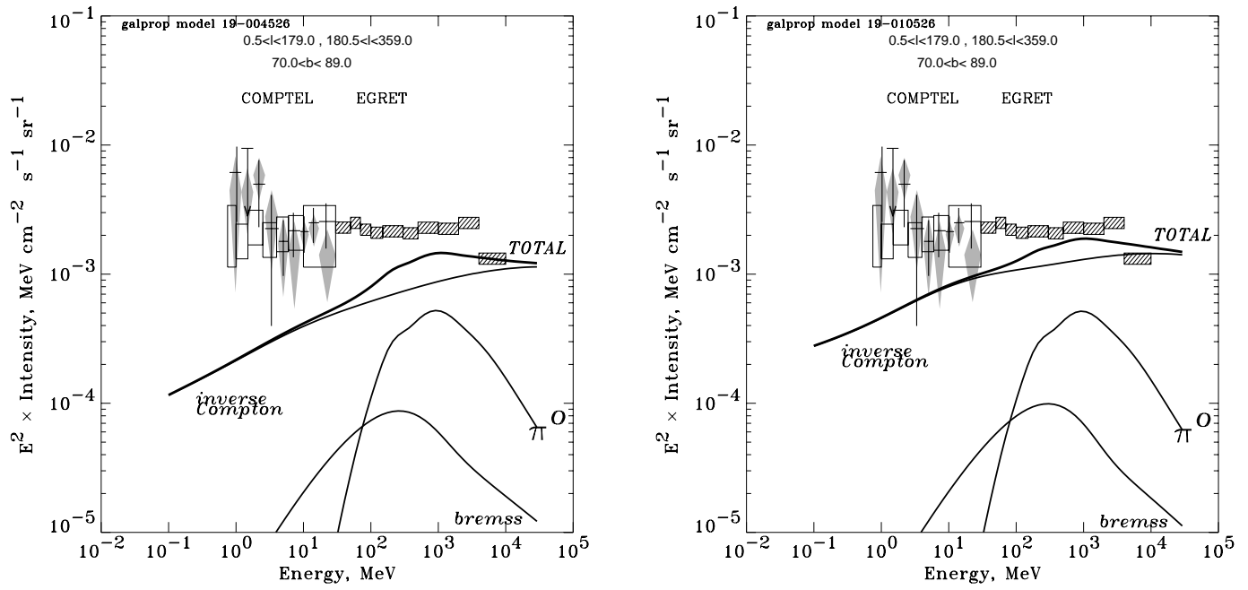
FIG. 18.—Energy spectrum of \gamma -rays from high Galactic latitudes ( |b| \geq 70^\circ , all longitudes) for HEMN model (left) and HELH model (right). Shaded areas show EGRET total intensity from Cycle 1–4 data. COMPTEL data: high-latitude total intensity (open boxes, Bloemen et al. 1999; diamonds, Kappadath 1998; crosses, Weidenspointner et al. 1999).
