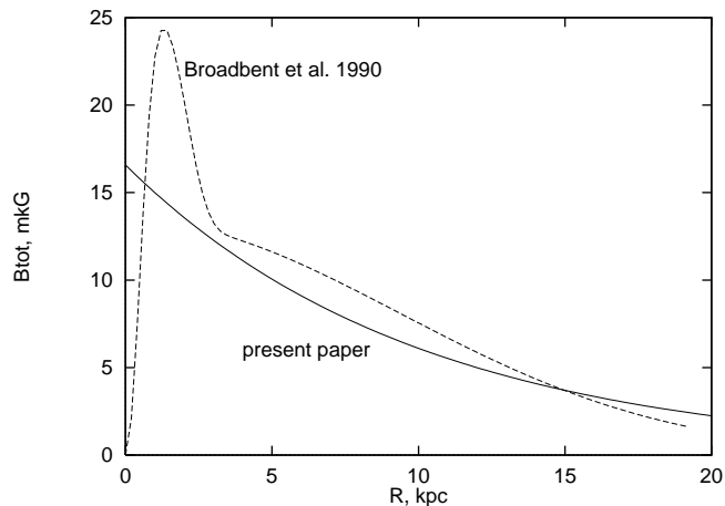
FIG. 6.—Magnetic field ( B_{\text{tot}} ) distribution at z=0 as used in our models (solid line) compared to parametrization by Broadbent et al. (1990) (dashed line).
