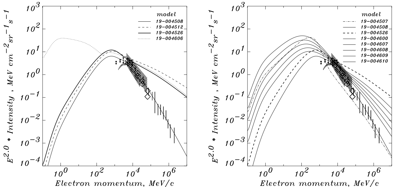
FIG. 2.—Electron spectra as obtained after propagation in our models compared with direct measurements. Data: Taira et al. (1993) (vertical lines); Golden et al. (1984, 1994) (shaded areas); Ferrando et al. (1996) (small diamonds); Barwick et al. (1998) (large diamonds). Left: Thin solid line, C model; dashed line, HE model; thick solid line, HEMN model; dotted line, SE model. Right: Electron injection spectral indices 2.0–2.4, no reacceleration.
