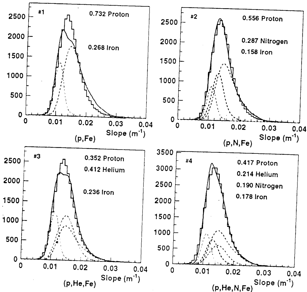
Fig. 8. A demonstration of the multi-species fitting procedure for the energy range 10^{14.9} - 10^{15.3} eV. The solid histogram gives the distribution of Cherenkov slope s for all CASA-BLANCA data in that energy range and is the same in all four panels. The solid curves show the combinations of Monte Carlo (QGSJET) showers which best reproduce the measured distribution. Panels 1–4 correspond to different combinations of primary species. Clearly, a nitrogen component is needed to match the data, but a helium component is also important.
