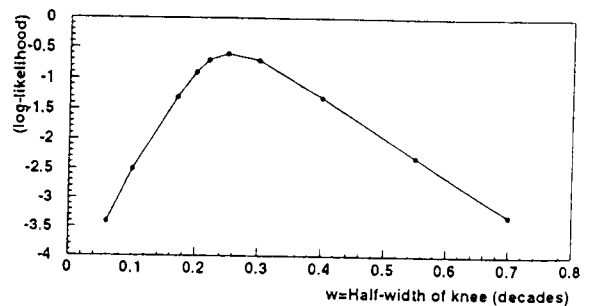
Fig. 3. Top: several trial functions used to fit the cosmic ray flux. Bottom: the log-likelihood for the smooth function at a range of widths w . The CASA-BLANCA data fit best to a knee with w = 0.25 or a full width of one-half decade.
