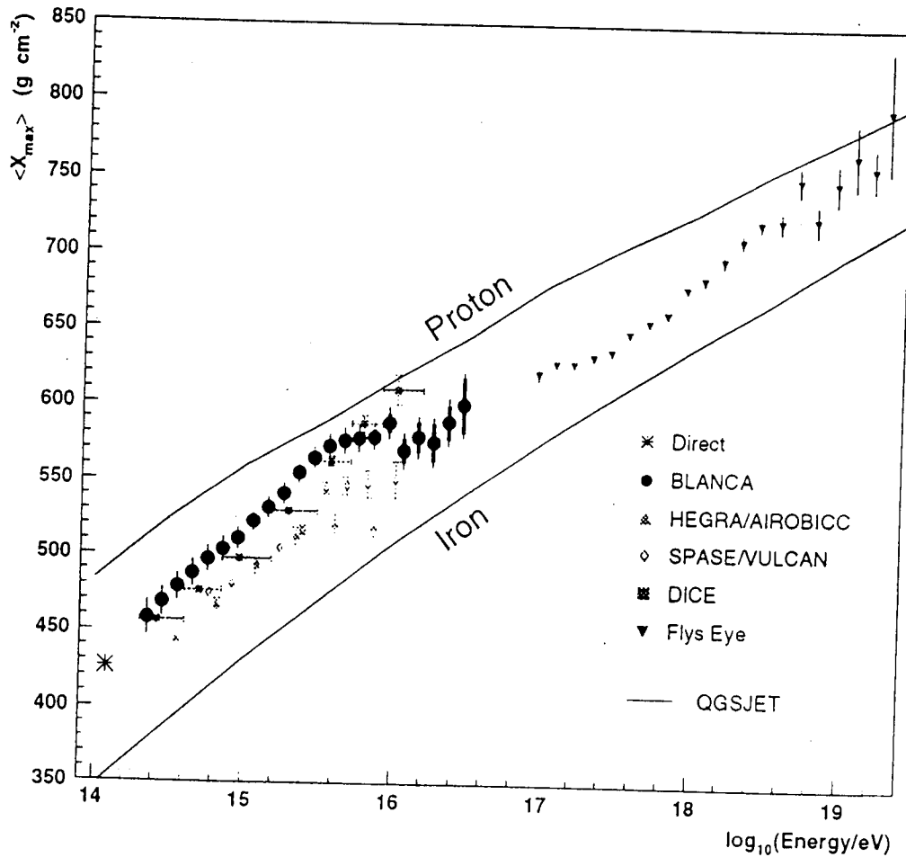
Fig. 10. The CASA-BLANCA measurement of X_{\max} compared with other results. All experiments operating near the knee use atmospheric Cherenkov light, including DICE [19], the AIROBICC array of HEGRA [8], and the VULCAN array at the South Pole [9]. The high energy measurements ( >10^{17} eV) by Fly's Eye use the atmospheric fluorescence technique [29]. The "direct" point estimates the mean X_{\max} that would be expected on the basis of direct balloon measurements [19]. The Monte Carlo lines use CORSIKA with QGSJET [30].
