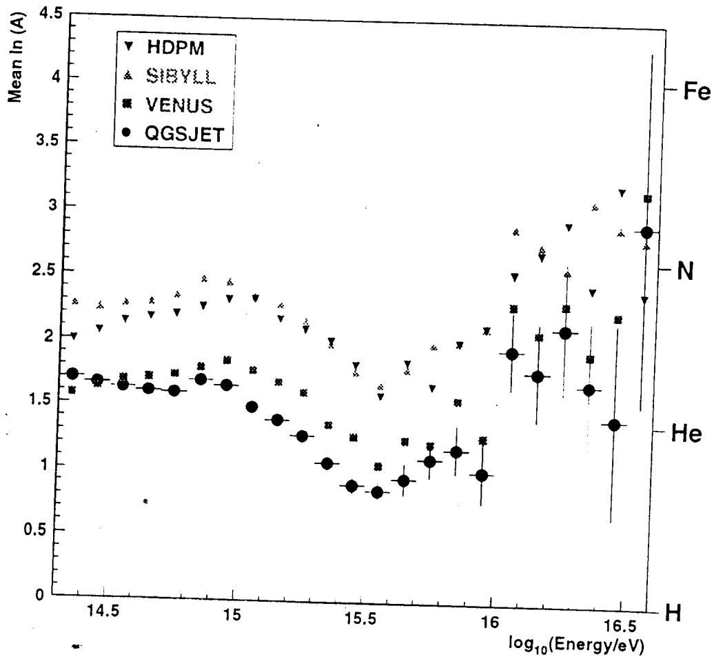
Fig. 7. The mean logarithmic mass ( \ln A ) measured by CASA-BLANCA as a function of energy. The four sets of symbols show the BLANCA data interpreted using CORSIKA coupled with the indicated hadronic interaction model. Error bars are statistical only and shown only on the QGSJET results; errors on the other points are of similar size. Assuming a hadronic model, the systematic uncertainties in the \ln A estimate are typically 0.2. The dominant systematic effect is clearly the difference between the hadronic models.
