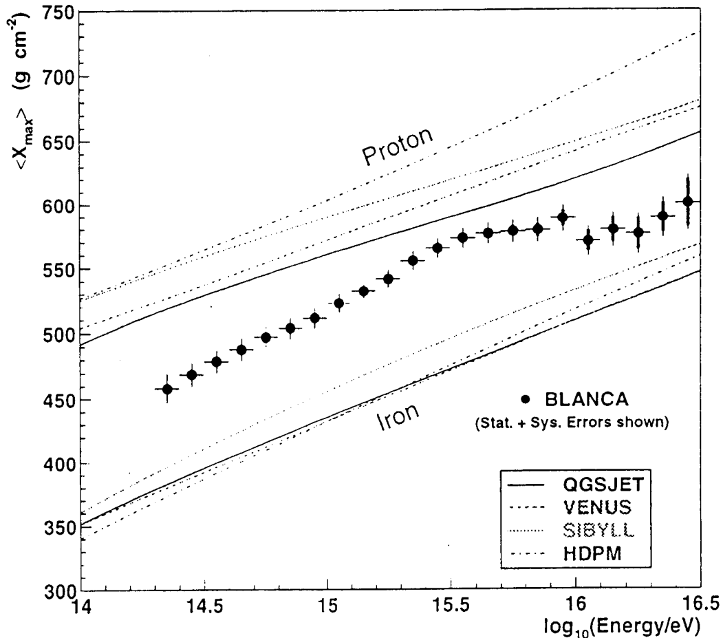
Fig. 5. The mean depth of shower maximum ( \langle X_{\max} \rangle ) measured by CASA-BLANCA as a function of energy. The lines represent the values for pure proton or pure iron samples predicted by each of the four hadronic interaction models. The thick error bars represent the statistical uncertainty, while the thin errors also include the systematic uncertainties discussed in the text; the former are important only above 10 PeV.
