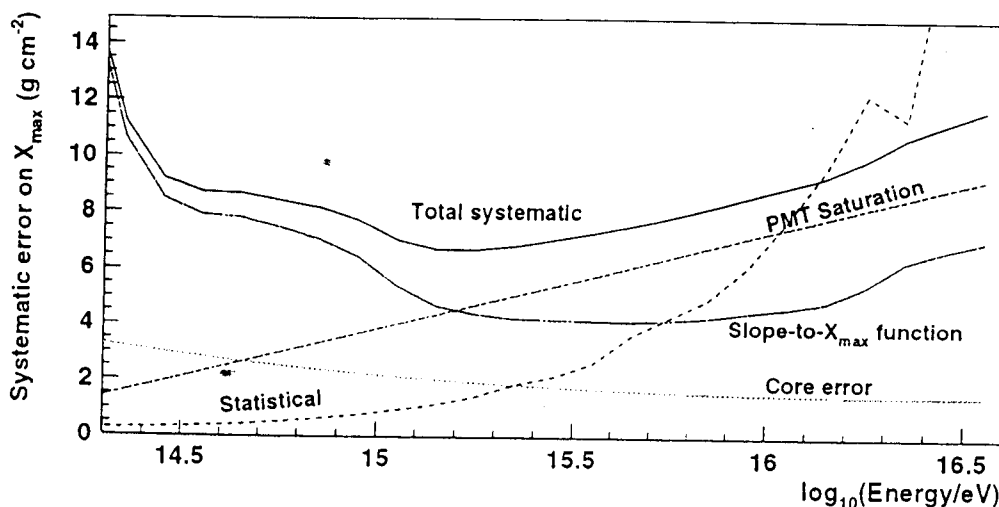
Fig. 6. Systematic uncertainties on CASA-BLANCA X_{\max} estimates. At low energies, the dominant error comes from the slope-to- X_{\max} conversion function; at high energies, the uncertain photomultiplier linearity is more important. For comparison, the statistical error on the CASA-BLANCA mean X_{\max} measurements is also shown (---), assuming a bin width of 0.1 decades.
