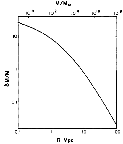
FIG. 1.—The rms fluctuation in the mass found within a sphere of radius R . The top scale is the mean mass within the sphere. The vertical normalization is adjusted to make \delta M/M agree with the observed fluctuation, \delta N/N , in the count of bright galaxies at R = 8 h^{-1} Mpc. This curve is based on the assumptions that the universe is dominated by very massive, weakly interacting particles and that the initial density fluctuations were adiabatic with power spectrum P \propto k .
