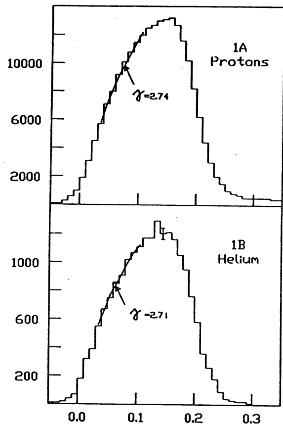
Figure 1. Deflection spectra
