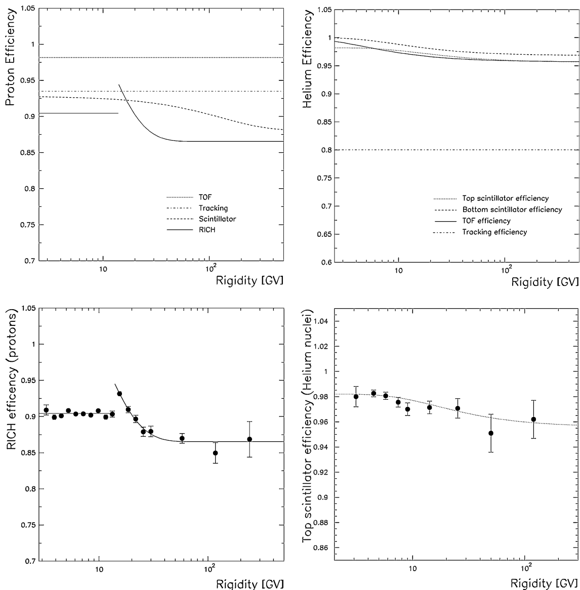
Fig. 6. First row: selection efficiencies as a function of rigidity for protons (left) and helium nuclei (right). The total efficiency, not shown in figures, is the product of the different functions. Second row, two examples of efficiency determination: the RICH selection efficiency for proton (left) and the top scintillator efficiency for helium nuclei (right).
