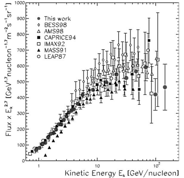
Fig. 11. The helium energy spectrum at the top of atmosphere detected by CAPRICE98. Results from other recent experiments are also shown: BESS98 [4], AMS98 [5], CAPRICE94 [3], IMAX92 [8], MASS91 [7], LEAP87 [6].
