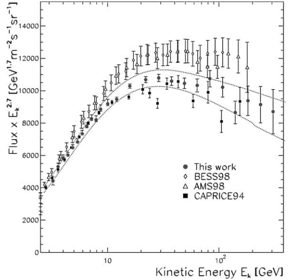
Fig. 12. The proton energy spectrum at the top of atmosphere detected by CAPRICE98. The upper and lower limit for the estimated systematic errors, described in Section 3.7, are shown as dotted lines; they include an offset in the deflection measurement of 7 \times 10^{-4} \text{ GV}^{-1} . The error bars represent the statistical errors plus the systematics due to efficiencies (Section 3.2), see Table 4. Results from BESS98, AMS98 and CAPRICE94 experiments are also shown.
