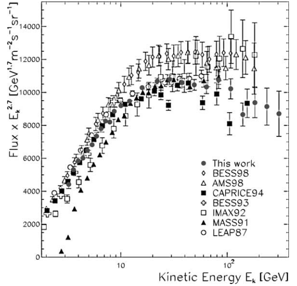
Fig. 10. The proton energy spectrum at the top of atmosphere detected by CAPRICE98. Results from other recent experiments are also shown: BESS98 [4], AMS98 [5], CAPRICE94 [3], BESS93 [38], IMAX92 [8], MASS91 [7], LEAP87 [6].
