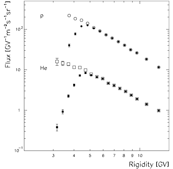
Fig. 8. Effects of the geomagnetic transmission correction on the proton and helium nuclei fluxes. Solid symbols represent the fluxes without correction while open symbols are fluxes after the correction.
