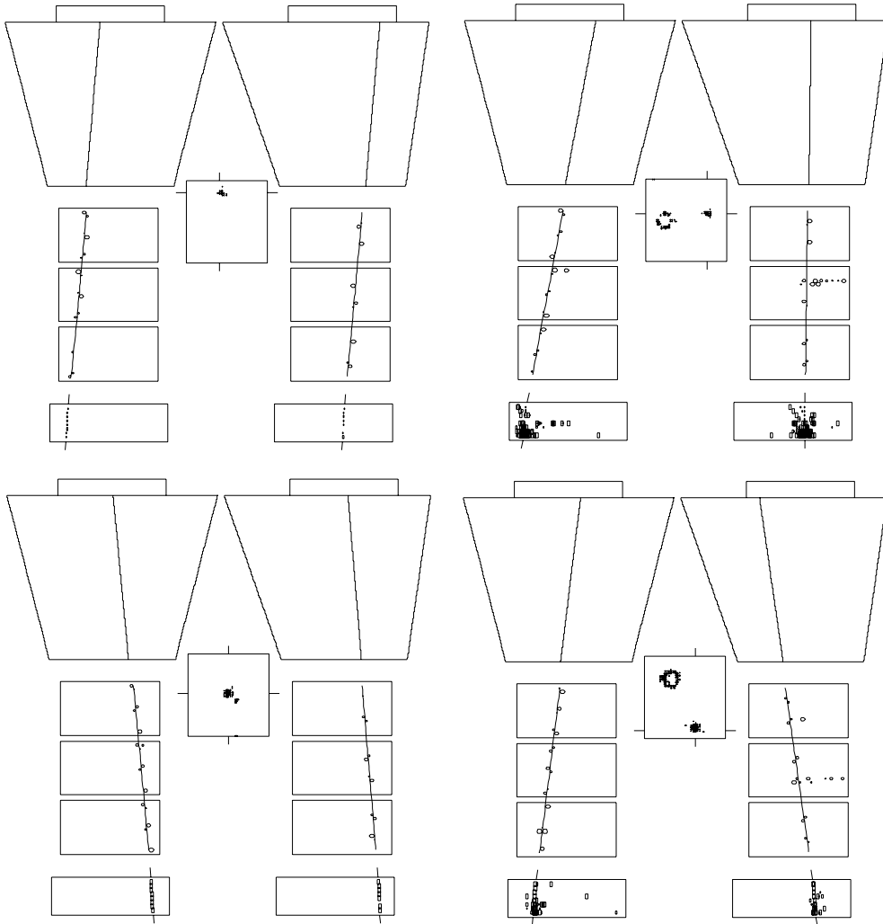
Fig. 3. Display of two protons and two helium nuclei traversing the CAPRICE98 apparatus. Clockwise from the upper left: a 5.6 GV non-interacting proton, in the RICH only a ionization cluster is visible; a 37.8 GV interacting proton, the ionization cluster of pads can be seen well separated from the Cherenkov ring; an 82.5 GV interacting helium, notice that the ionization and Cherenkov energy released in the RICH is higher than for a singly charged particle; a 26.7 GV non-interacting helium, note the signature of a helium nucleus in the calorimeter, where the size of the square is proportional to the detected energy: the ionization loss energy released is four time higher with respect to the case of a proton.
