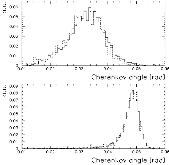
Fig. 9. The Cherenkov angle distribution in the rigidity bin from 21.4 to 22.9 GV is shown at the top, while at the bottom is shown for a bin from 40.5 to 53.4 GV; here, the dashed lines are for real data and solid lines are for simulated data.
