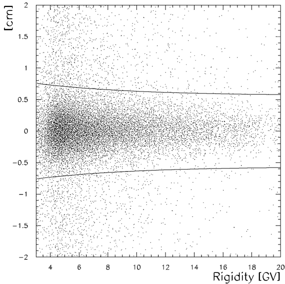
Fig. 5. The difference between the particle impact position on the paddle plane as determined by the RICH and the tracking system is shown as function of rigidity (in the case of the x view for a sample of about 30,000 events); the events between the two lines, representing the 3\sigma limits, were selected.
