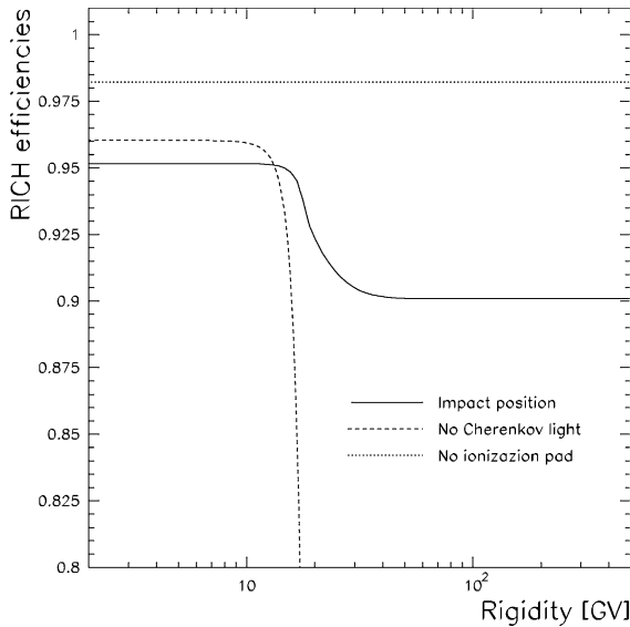
Fig. 7. Proton selection efficiencies as a function of rigidity for the RICH. Since the “no-ionization” and the “impact position” conditions are correlated the total efficiency for the RICH is higher than the product of the three partial efficiencies.
