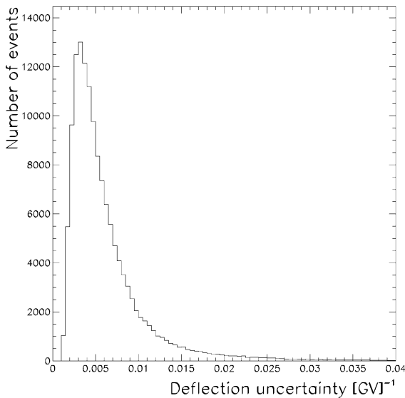
Fig. 2. Distribution of the deflection uncertainty for protons.
