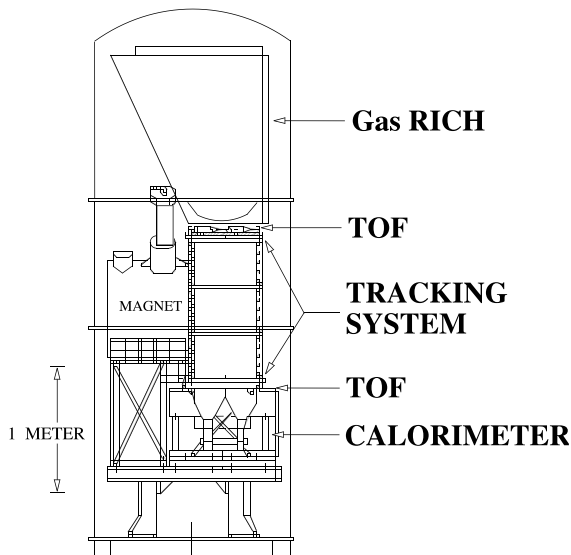
Fig. 1. The CAPRICE apparatus in the 1998 configuration (CAPRICE98).
