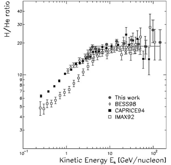
Fig. 13. Proton to helium nuclei flux ratio at the top of the atmosphere as a function of kinetic energy per nucleon. Results from other recent experiments are also shown: BESS98 [4], CAPRICE94 [3], IMAX92 [8].
