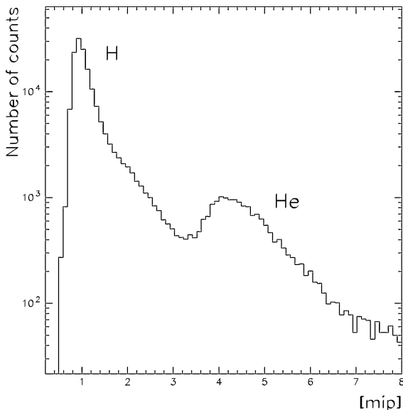
Fig. 4. The pulse-height spectrum, top scintillator, for a sample of events; both the singly charged particles and the helium nuclei peaks can be easily identified.
