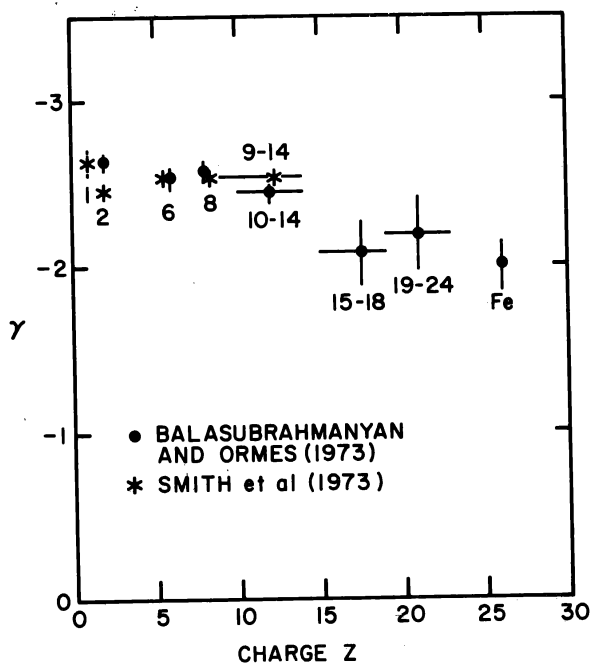
Figure 1. Exponents of Energy Spectra vs. Charge
