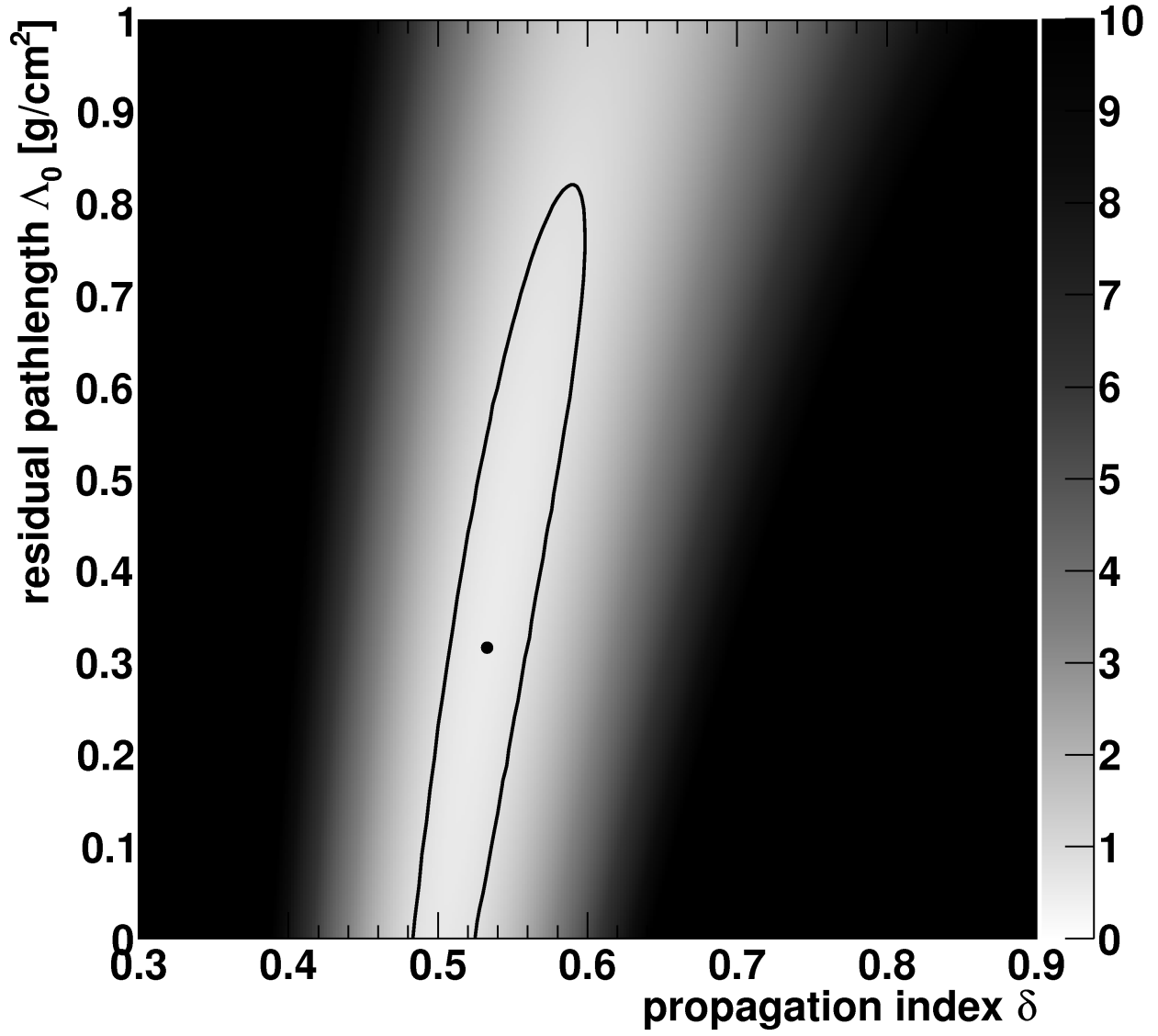
Fig. 3.— \chi^2 map in the parameter space of \delta vs. \Lambda_0 for the Leaky-Box model fit to TRACER data. The best fit values are marked at (\delta, \Lambda_0) = (0.53 \pm 0.06, 0.31^{+0.55}_{-0.31} \text{ g cm}^{-2}) and the 1\sigma contour is indicated.
