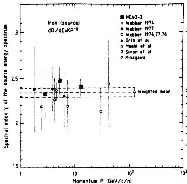
Fig. 3 : Iron source spectral index plotted as a function of momentum, assuming for the spectral shape a power law in momentum.
