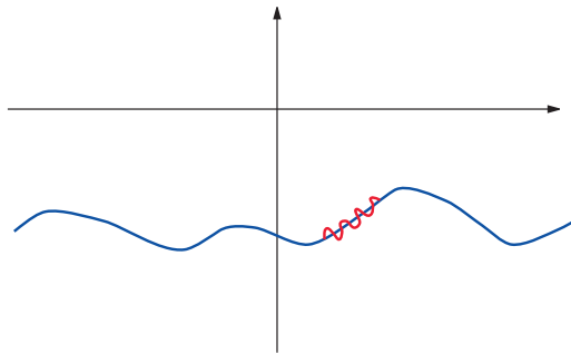
Fig. 2. Due to the perturbations of the radial field, the evolution of phase perturbations proceeds in inhomogeneous background that slowly varies in space.
