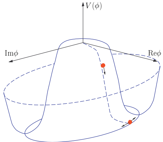
Fig. 1. The scalar potential in the pseudo-Nambu–Goldstone scenario.
