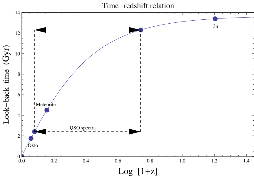
Figure 1: (Top): Summary of the systems that have been used to probe the constancy of the fundamental constants and their position in a space-time diagram in which the cone represents our past light cone. The shaded areas represents the comoving space probed by different tests. (Bottom): The look-back time-redshift relation for the standard \Lambda CDM model.
