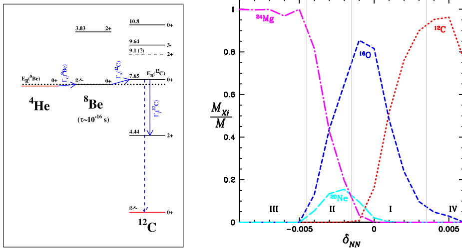
Figure 5: (Left) Level scheme of nuclei participating to the {}^4\text{He}(\alpha\alpha, \gamma){}^{12}\text{C} reaction. (Right) Central abundances at the end of the CHe burning as a function of \delta_{NN} for a 60M_\odot star with Z = 0 . From Ref. [103].
