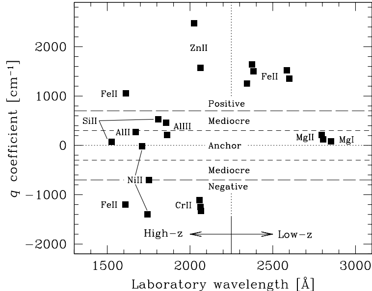
Figure 3: Summary of the values of some coefficients entering the parameterization (69) and necessary to interpret the QSO absorption spectra data. From Ref. [370]
