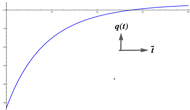
Figure 5: q(t) vs \tilde{t}
