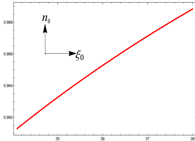
Figure 2: n_s vs \xi_0
