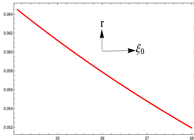
Figure 3: r vs \xi_0
