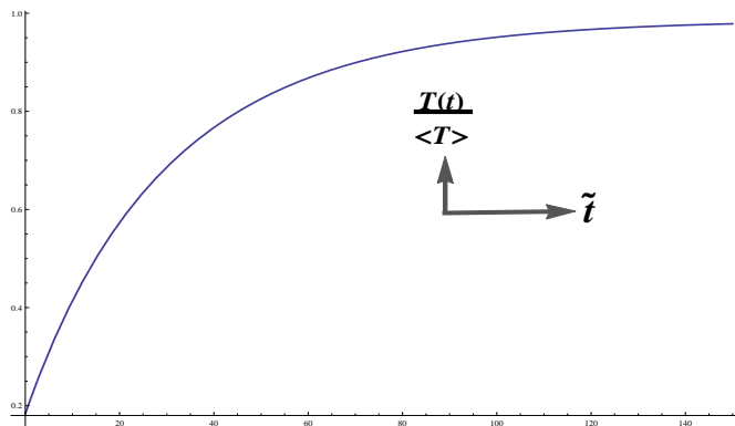
Figure 4: \frac{T(t)}{\langle T \rangle} vs \tilde{t}
