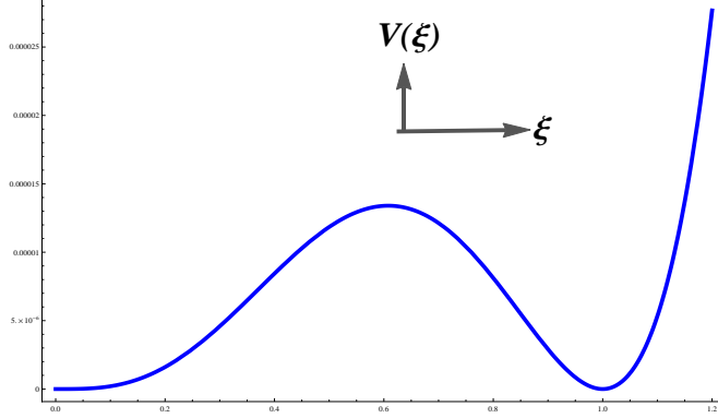
Figure 1: V(\xi) vs \xi
