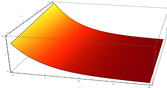
Figure 7: \chi^{(0)} vs \phi (along x axis) and t
