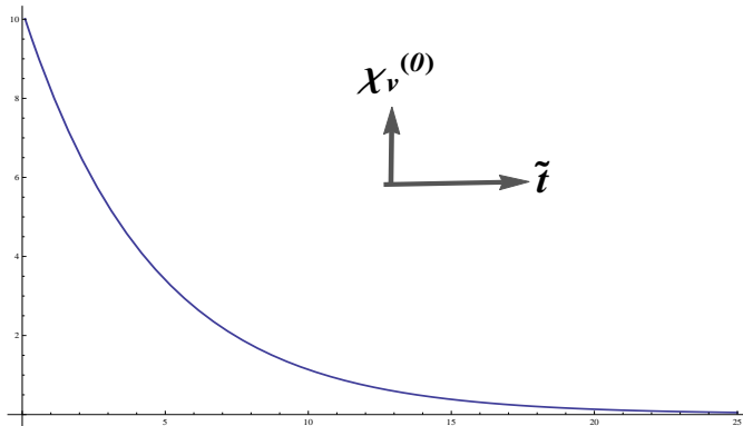
Figure 6: \chi_v^{(0)} vs \tilde{t}
