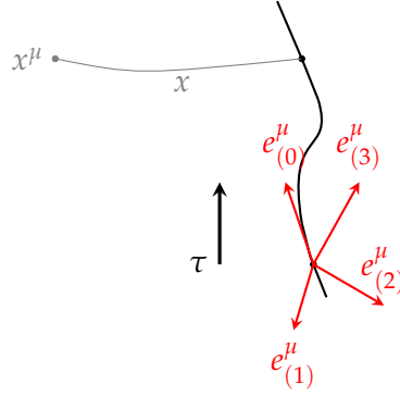
Figure 2.1.: z^\mu_{(\tau)} is the worldline of the observer and the adopted coordinates can be seen in red. One can see how to relate the neighbouring point x^\mu to this adopted coordinates. Note that x is the proper length of the geodesic connecting the worldline to the neighbouring point x^\mu .
