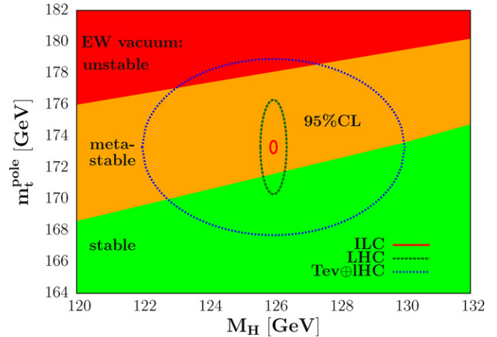
Fig. 1. The 2\sigma ellipses in the [M_H, m_t^{\text{pole}}] plane that one obtains from the current top quark and Higgs mass measurements at the Tevatron and LHC and which can be expected in future measurements at the LHC and at the ILC, when confronted with the areas in which the SM vacuum is absolutely stable, metastable and unstable up to the Planck scale.
