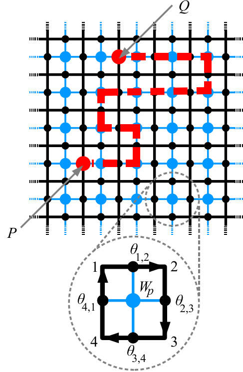
FIG. 1: (Color online) A 2D -dimensional rotor lattice. To every plaquette p is associated a rotor operator W_p as a function of the variables \theta_{ij} . The graph G is the one drawn in thin black lines. The graph G' is the graph with black and blue (lighter, bigger) dots as vertices and blue thin lines as edges. The red dashed line shows a path of length n = 22 from the point P to the point Q which are at a distance 2d(P, Q) = 8 on G' or d(P, Q) = 4 on G . These paths contain alternating link and plaquette operators.
