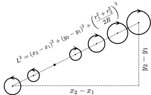
FIG. 3. Generalized Pythagoras theorem: Let L denote the geodesic distance between two loops, demonstrated here for circles of opposite sides, so that A_2 - A_1 = \pi(r_2^2 - (-r_1^2)) . While the shape of the loop stays unconstrained in the absence of loop dynamics, the center of mass location, as well as the loop area, evolve linearly.
