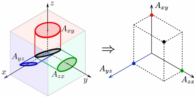
FIG. 2. Associated with every simple loop event (black) residing in an n -dim flat space or spacetime, there are \frac{1}{2}n(n-1) simple projected areas (red, blue, green,...), thereby mapping a loop event into a point \{A_{xy}, A_{yz}, A_{zx}, \dots\} in loop space.
