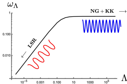
FIG. 5. High to low frequency transition as a function of the string tension \Lambda (plotted for the special case \ell = R = 1 ). While \omega_\Lambda is \Lambda -independent at the high- \omega regime, it is \sim \sqrt{\Lambda} at the low- \omega regime
