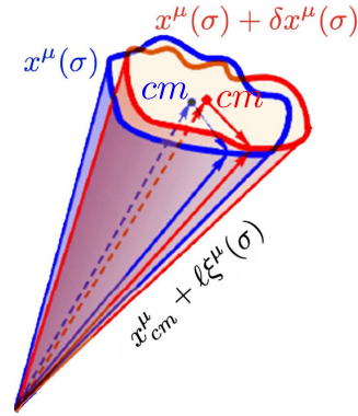
FIG. 1. Two neighbouring loops in spacetime are mapped into two infinitely closed points in loop spacetime. A tenable loop line element \delta S must then reproduce, at the shrinking loop limit \ell \rightarrow 0 , the special/general relativistic line element measuring the distance between the two infinitely separated center-of-masses, respectively.
