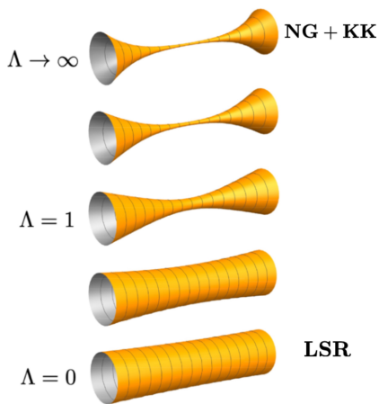
FIG. 4. From LSR to NG+KK: Soap branes connecting two identical circular rings, residing in a 3-dim space and separated 2h apart. As \Lambda grows, while holding the KK radius R fixed, the LSR cylinder transforms into an NG+KK narrow waist candlestick (owing its stability to R \neq 0 ).
