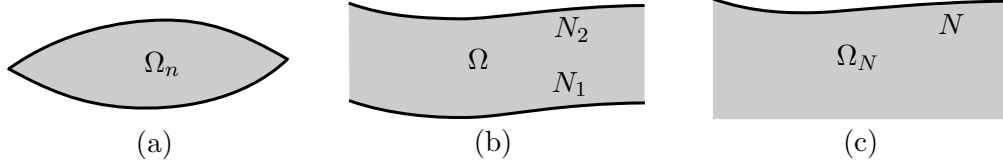
FIGURE 9.2. Choices of spacetime regions: Lens-shaped region (a), region between two Cauchy surfaces (b) and past of a Cauchy surface (c).
