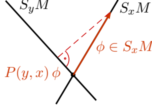
FIGURE 5.8. The kernel of the fermionic projector
