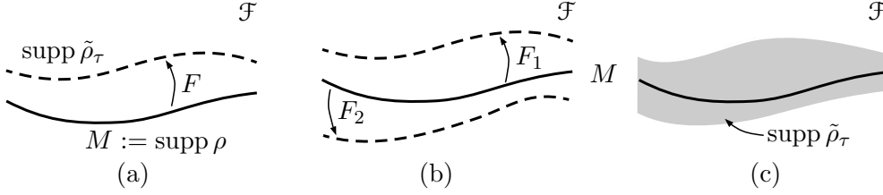
FIGURE 8.1. Illustration of the fragmentation of the measure \rho : Smooth variation (a), disintegration into two components (b) and general enlargement of the support (c).
