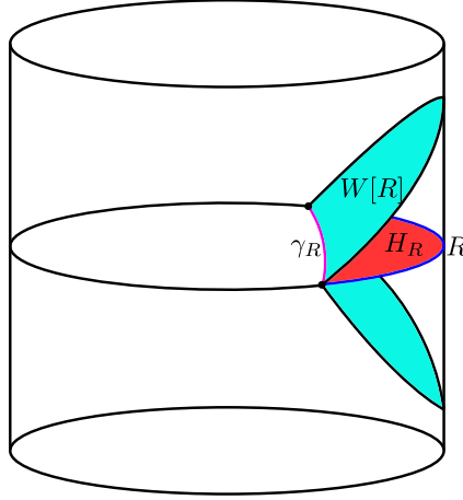
Figure 23: The HRT surface \gamma_R and entanglement wedge W[R] of a boundary subregion R for AdS_3 . Here R extends between the two black dots, and is shaded blue. \gamma_R is shaded purple, a homology hypersurface H_R is shaded red, and W[R] is the spacetime volume between the two light blue surfaces.
