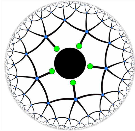
Figure 22: A tensor network black hole. One “effective field theory” index is replaced by five new “black hole microstate” indices, shaded green.
