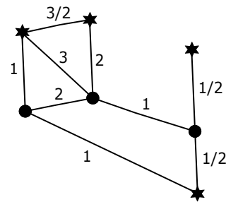
Figure 1. Exemplary generalised spin network state. Vertices with a spin \frac{1}{2} particle are depicted by stars and vertices without matter by dots. The spin \frac{1}{2} particles couple to the star intertwiner gauge invariantly. For the sake of clarity, arrows depicting the direction of the edges are omitted.
