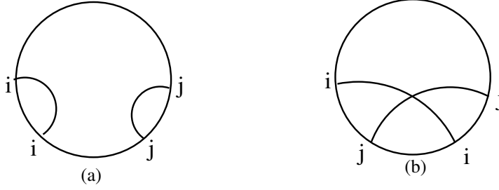
Figure 10: Two configurations for the fermions. In (a) we have the ii jj configuration with \chi < 1 and on the right we have the ijij configuration with \chi > 1 .
