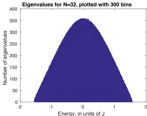
Figure 13: The spectrum for a single realization of the q = 4 model with N = 32 fermions.
