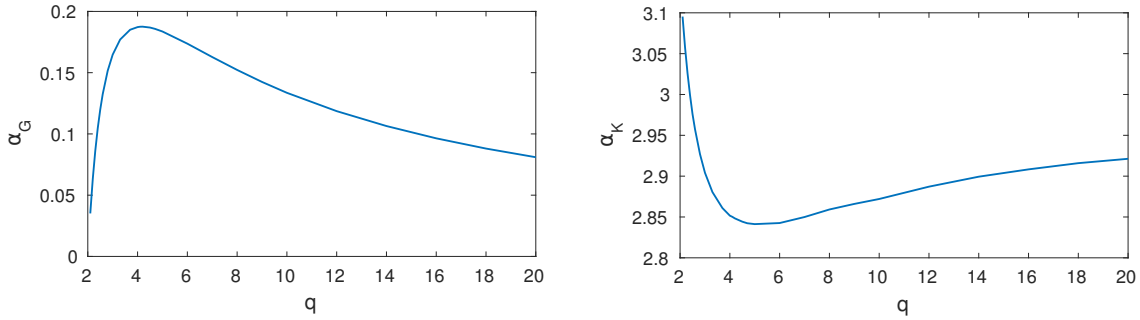
Figure 9: The functions \alpha_G(q) and \alpha_K(q) , computed by solving the Schwinger Dyson equations numerically for different values of q . The first three physical values are \alpha_G(2) = 0 , \alpha_G(4) \approx 0.1872 , and \alpha_G(6) \approx 0.1737 . Analytically, we know that \alpha_G behaves as 2/q at large q , and like \pi(q-2)/8 for q near two. \alpha_K never strays more than roughly five percent from the large q value of three.
