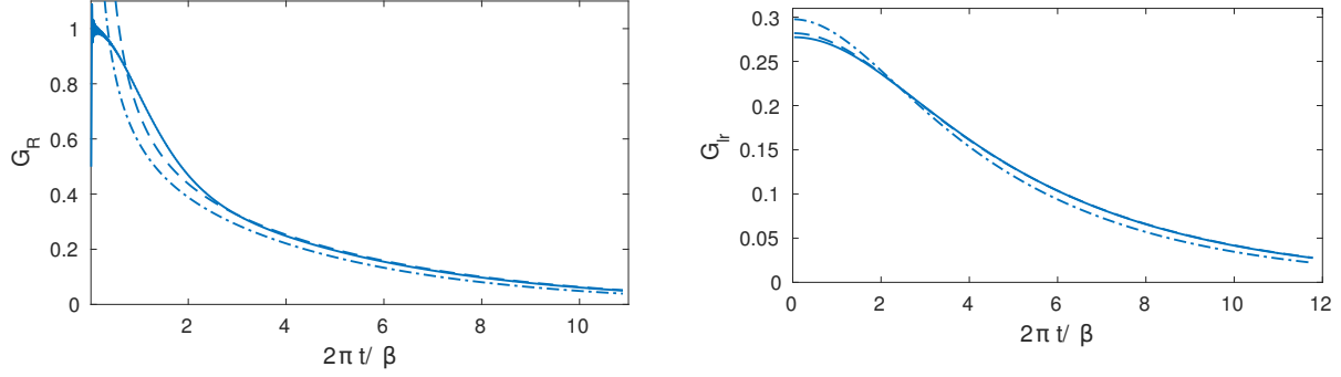
Figure 16: The retarded propagator G_R (left) and the half-circle Wightman correlator G_{lr} (right) are plotted in the q = 4 model with \beta J = 10 . The solid curve is the numerical answer, the dash-dotted curve is the conformal answer, and the dashed curve is the conformal answer plus the leading correction (3.161). The behavior of the numerical G_R near t = 0 is somewhat contaminated by finite-cutoff wiggles.
