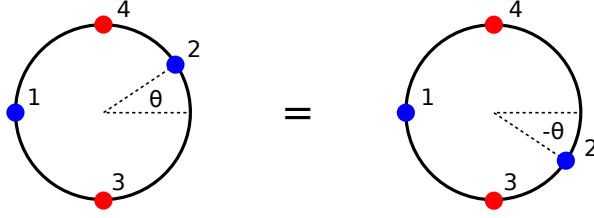
Figure 5: The symmetry of the \chi > 1 correlator under \chi \rightarrow \frac{\chi}{\chi-1} is manifest as \theta \rightarrow -\theta after mapping to the circle.
