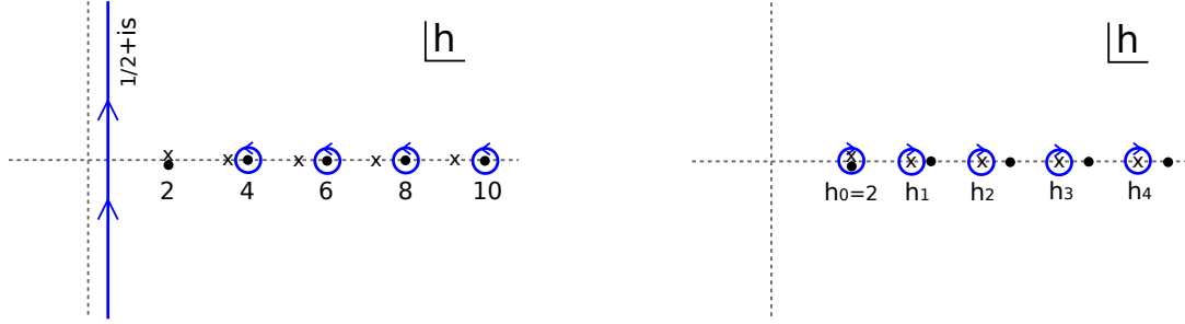
Figure 7: The continuum piece of the contour that defines \mathcal{F}_{h \neq 2} can be pushed to the right, canceling the residues of the poles of the 1/\tan(\pi h/2) (dots), and picking up poles from the locations where k_c(h) = 1 (crosses). We have a double pole at h = 2 .
