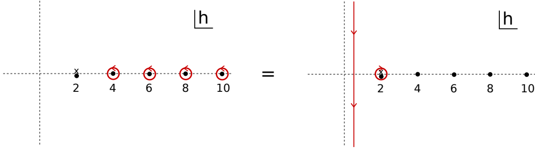
Figure 8: To continue the sum over residues to the chaos region, we first replace the k_c(h) by k_R(1-h) , and then pull the contour surrounding the poles back to the line 1/2 + is , picking up the double pole at h = 2 but no other poles. In this form the function can safely be continued. In addition we also have the original integral along h = 1/2 + is with the function k_c ; we leave this piece alone because it can already be continued.
