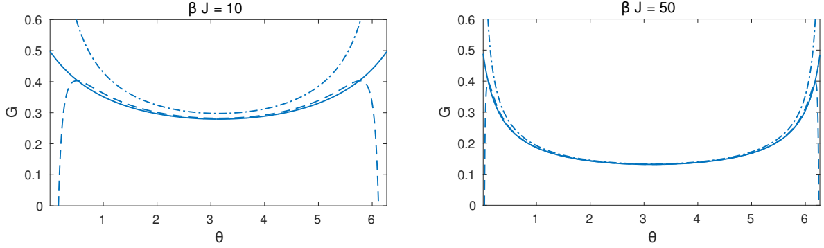
Figure 15: The exact G(\theta) in the q = 4 model is shown in solid lines, for \beta J = 10 (left) and \beta J = 50 (right). We also plot the conformal answer G_c in dash-dotted lines, and the conformal answer plus the first correction G_c f_0 in dashed lines.
