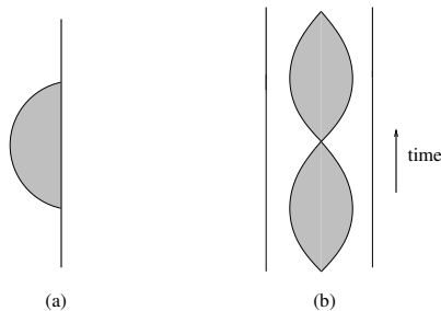
Figure 14: (a) Particle with a string going to the boundary. (b) Pair of particles in the bulk with a string connecting them. They are oscillating in global AdS_2 . We can view the string as fundamental or as a color electric flux of an O(N) gauge field.
