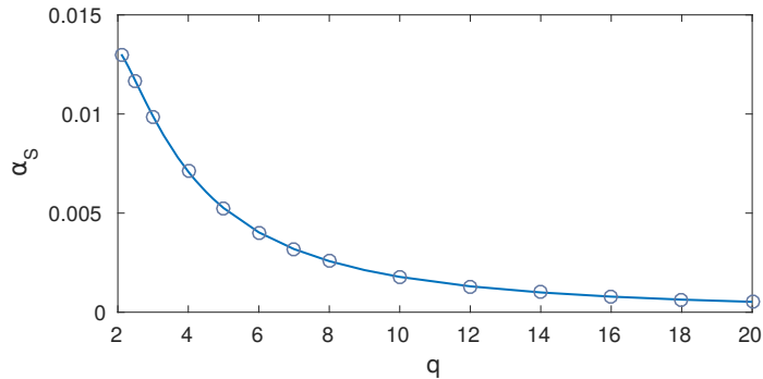
Figure 12: The coefficient of the Schwarzian action \alpha_S is plotted. The blue curve is the value given by the previously computed \alpha_G . The circles are values inferred from (5.181) and the numerical evaluation of the specific heat c . The agreement is a check that the Schwarzian action is correct nonlinearly, not just for small reparameterizations.
