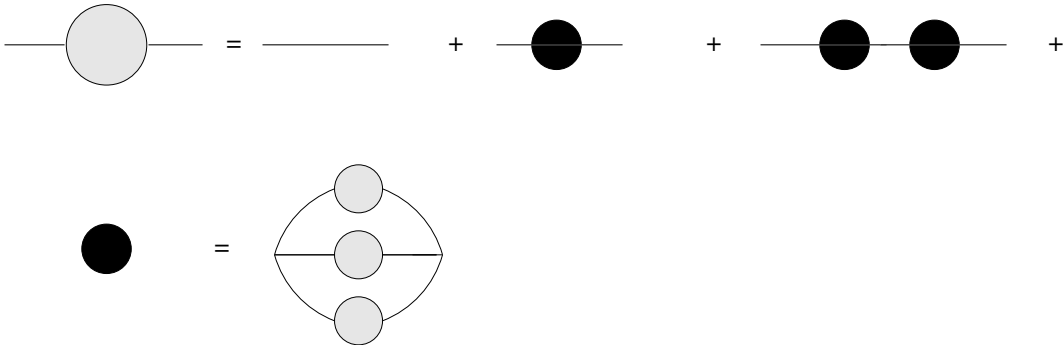
Figure 2: Equations that define the summation of the leading large N contributions, for the q = 4 case. The solid circle represents the one particle irreducible contributions. The dotted circle represents the full two point function. This is a graphical representation of the equations in (2.6).
