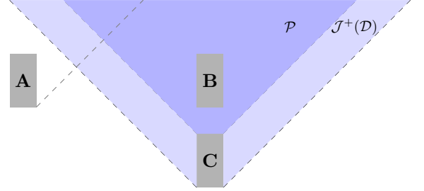
FIG. 1. Configuration in a slice of spacetime of the interaction regions of detectors A, B and C. In blue, the causal future of the projective measurement performed on C, \mathcal{P} ; in pale blue, the causal future of the measurement that is not already in the future of the projective measurement, \mathcal{J}^+(\mathcal{D}) \setminus \mathcal{P} .
