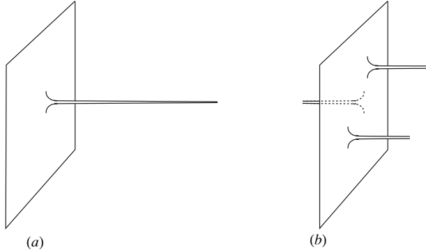
Fig. 5.1. The D -dimensional interpretation of the BIon solution. (a) It is an infinitely long spike representing a fundamental string ending on the D -brane. (b) BIONS are BPS and therefore can be added together at no cost to make a multi-BIon solution.
