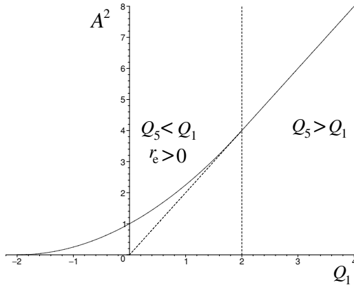
Fig. 17.2. The square of the maximal horizon area as a function of Q_1 , for fixed Q_P (=1) and Q_5 (=2) . For N_1 > 2N_5 , the (\text{area})^2 increases linearly. For N_1 < 2N_5 , to maximise the area, one must use only N_1/2 of the available D5-branes (see figure 17.1), and therefore the dependence on N_1 is quadratic.
