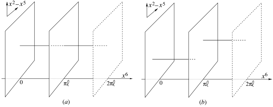
Fig. 13.4. (a) This configuration of two NS5-branes on a circle with D2-branes stretched between them is dual to a D1-brane probing an A_1 ALE space. (b) The Coulomb branch where the D2-brane splits into two ‘fractional branes’.
