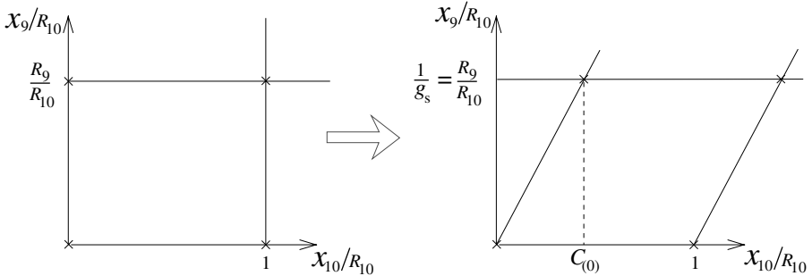
Fig. 16.9. Generalising the compactification lattice by including a shift. This is how the F-theory or type IIB theory torus arises from M-theory.
