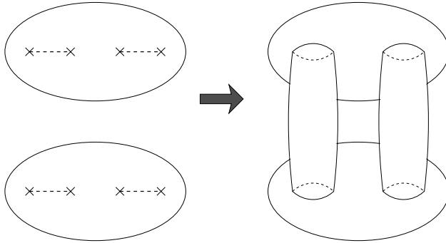
Fig. 16.2. Why a cubic gives a torus.
