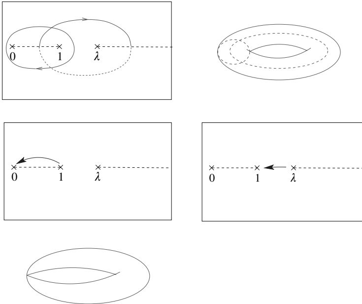
Fig. 16.4. The top sketches show one sheet of the cut complex x plane and the generic torus made from it, including the two classes of one-cycle (cf. figure 16.2). (Note that the dotted half of one of the curves is in fact on the other sheet.) The bottom sketches show how the torus can degenerate if roots collide, giving \Delta = 0 (cf. figure 16.3).
