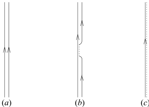
Fig. 11.1. (a) A parallel D-string and F-string, which is not supersymmetric. (b) The F-string breaks, its ends attaching to the D-string, resulting in (c) the final supersymmetric state, a D-string with flux.
