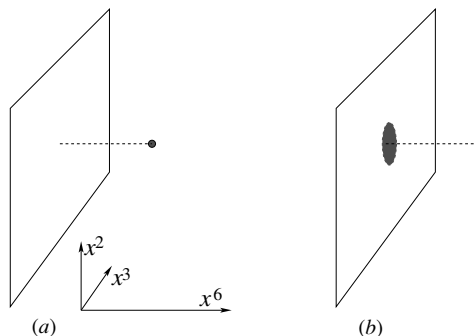
Fig. 13.7. Instantons and the Dp - D(p+4) system. (a) The Coulomb branch of the Dp -brane theory represents a pointlike brane away from the D(p+4) -brane. (b) The Higgs branch corresponds to it being stuck inside the D(p+4) -brane as a finite sized instanton of the D(p+4) -brane's gauge theory.
