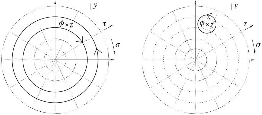
Fig. 3.1. Computing the commutator between the generator Q , defined as a contour in the y -plane, and the operator \phi , inserted at z . The result in the limit y \rightarrow z is on the right.
