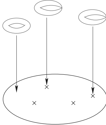
Fig. 16.5. The F-theory description of 24 sevenbranes (located at the crosses) as a torus fibration of T^2 over \mathbb{CP}^1 . In fact, this is a description of K3 as an elliptic fibration!
