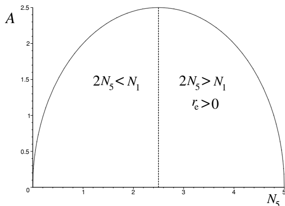
Fig. 17.1. The horizon area as a function of N_5 , for fixed Q_P (= 1) and N_1 (= 5) , which forms half of an ellipse. As the number of D5-branes increases past N_1/2 , the area decreases.
