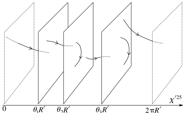
Fig. 4.3. Three D-branes at different positions, with various strings attached.
