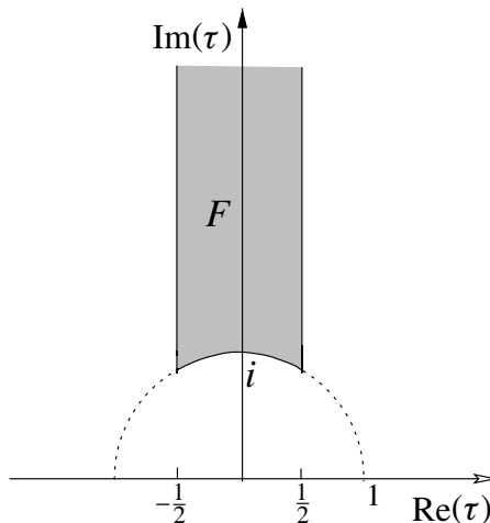
Fig. 3.3. The space of inequivalent tori.
