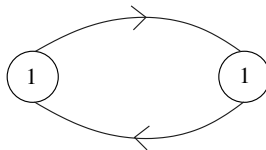
Fig. 13.1. A diagram showing the content of the probe gauge theory. The nodes give information about the gauge groups, while the links give the amount and charges of the matter hypermultiplets.
