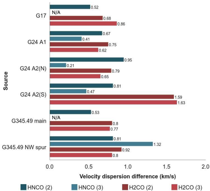
Fig. 15. Average velocity dispersion difference between NH 2 CHO and transitions HNCO (2) and (3) and H 2 CO (2) and (3). For the G24 sources HNCO (1) is used instead of HNCO (2).
