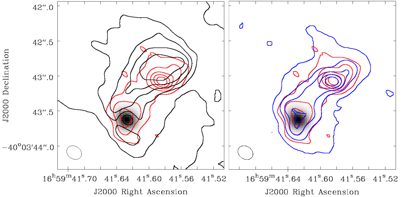
Fig. 6. G345 zeroth moment maps (contours) overlaid on the dust continuum (grayscale). Left: the black contours show the \text{H}_2\text{CO} (3) transition ( E_{\text{up}}=68.1 K) from 5\sigma to a peak of 0.402 Jy/beam \text{km s}^{-1} (contour levels 0.027, 0.102, 0.177, 0.232, and 0.327 Jy/beam \text{km s}^{-1} ). The red contours show \text{NH}_2\text{CHO} (1) emission ( E_{\text{up}}=60.8 K) from 5\sigma to 0.242 Jy/beam \text{km s}^{-1} (contour levels 0.020, 0.064, 0.109, 0.153, and 0.198 Jy/beam \text{km s}^{-1} ). Right: the blue contours show the extent of the \text{HNC} (2) emission ( E_{\text{up}}=101.5 K) from 5\sigma to 0.428 Jy/beam \text{km s}^{-1} (contour levels 0.014, 0.097, 0.180, 0.262, and 0.345 Jy/beam \text{km s}^{-1} ) with the red contours showing \text{NH}_2\text{CHO} (as in the left frame).
