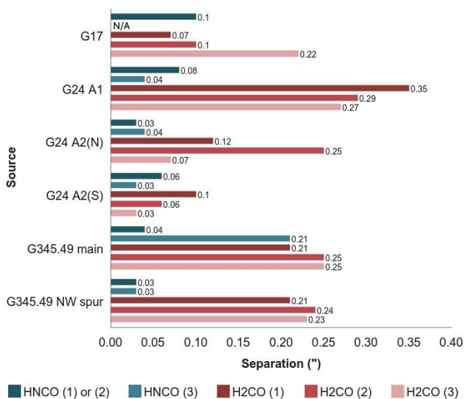
Fig. 7. Separations between NH 2 CHO and each peak of HNCO and H 2 CO. For the G24 sources HNCO (1) is used instead of HNCO (2) (see Table 3). The error in the peak position is \sim 0.01'' .
