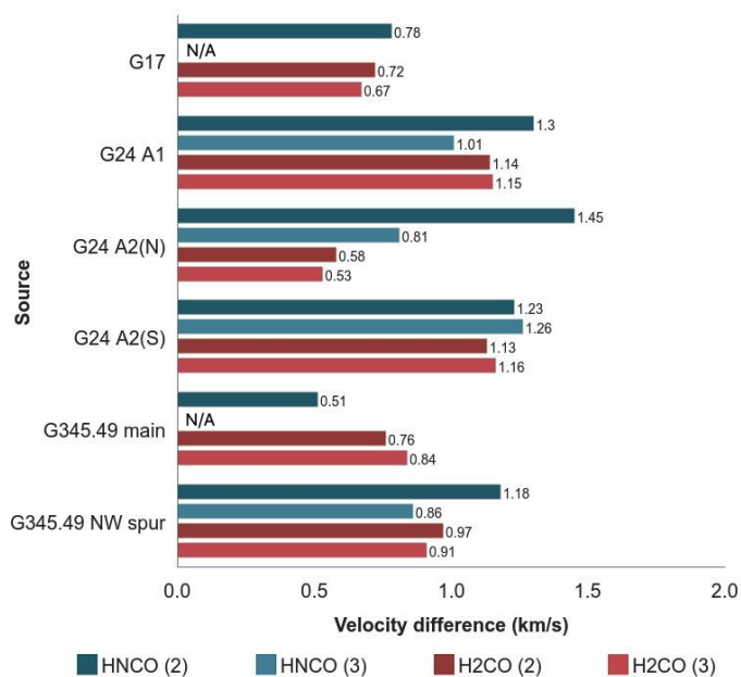
Fig. 11. Average velocity difference between \text{NH}_2\text{CHO} and transitions \text{HNCO} (2) and (3) and \text{H}_2\text{CO} (2) and (3). For the G24 sources \text{HNCO} (1) is used instead of \text{HNCO} (2) (see Table 3).
