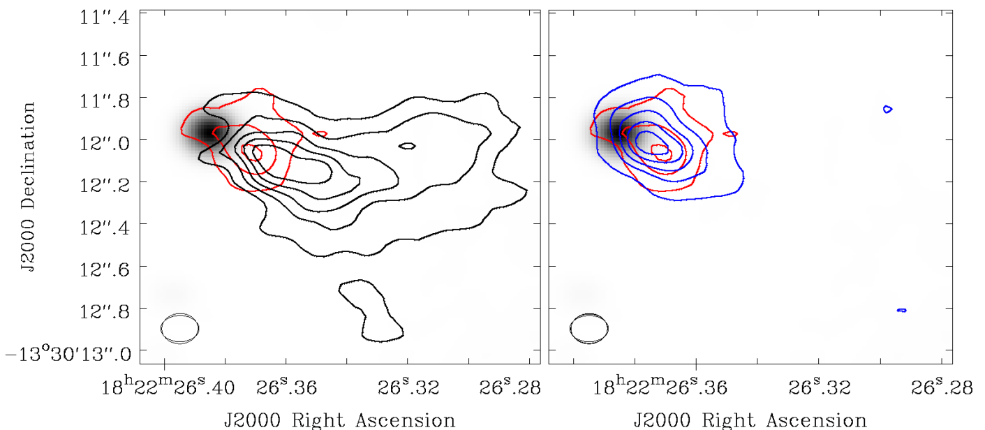
Fig. 4. G17 zeroth moment maps (contours) overlaid on the dust continuum (grayscale). Left: the black contours show the \text{H}_2\text{CO} (2) transition ( E_{\text{up}}=68.1 K) from 5\sigma to a peak of 0.175 Jy/beam \text{km s}^{-1} (contour levels 0.021, 0.052, 0.083, 0.113, and 0.144 Jy/beam \text{km s}^{-1} ). The red contours show \text{NH}_2\text{CHO} (1) emission ( E_{\text{up}}=60.8 K) from 5\sigma to 0.268 Jy/beam \text{km s}^{-1} (contour levels 0.022, 0.071, 0.120, 0.170, and 0.219 Jy/beam \text{km s}^{-1} ). Right: the blue contours show the extent of the \text{HNC} (2) emission ( E_{\text{up}}=101.5 K) from 5\sigma to 0.146 Jy/beam \text{km s}^{-1} (contour levels 0.010, 0.037, 0.064, 0.092, and 0.119 Jy/beam \text{km s}^{-1} ) with the red contours showing \text{NH}_2\text{CHO} (as in the left frame).
