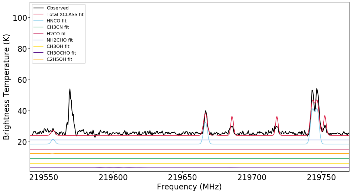
Fig. B.11. Spectral window from 219.5-219.8 GHz for G345 NW containing HNC (3). The additional transitions shown in the total XCLASS fit are \text{HC}_3\text{N} (219675 MHz), \text{C}_2\text{H}_5\text{CN} (219699 MHz), and \text{CH}_3\text{CHO} (219756 MHz).
