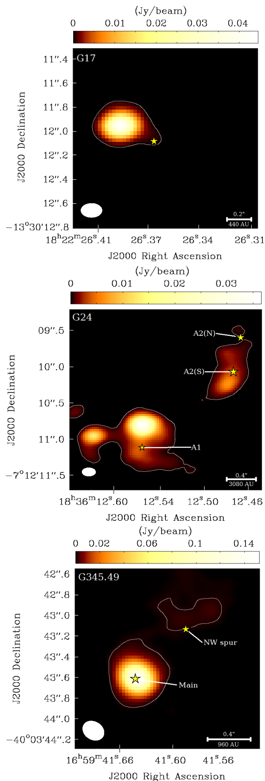
Fig. 1. Images of the 218 GHz continuum emission from Cycle 2 ALMA observations of our three regions focusing on the regions where \text{NH}_2\text{CHO} emission is observed. The color scale indicates the continuum flux as detailed in the color bar above each map. The white contour shows the 5\sigma contour levels for each panel: 1.5, 2.5, and 2.5 mJy/beam. The stars mark each of the spectral extraction points (coinciding with the zeroth moment peaks of \text{NH}_2\text{CHO} emission) and subsources are labeled.
