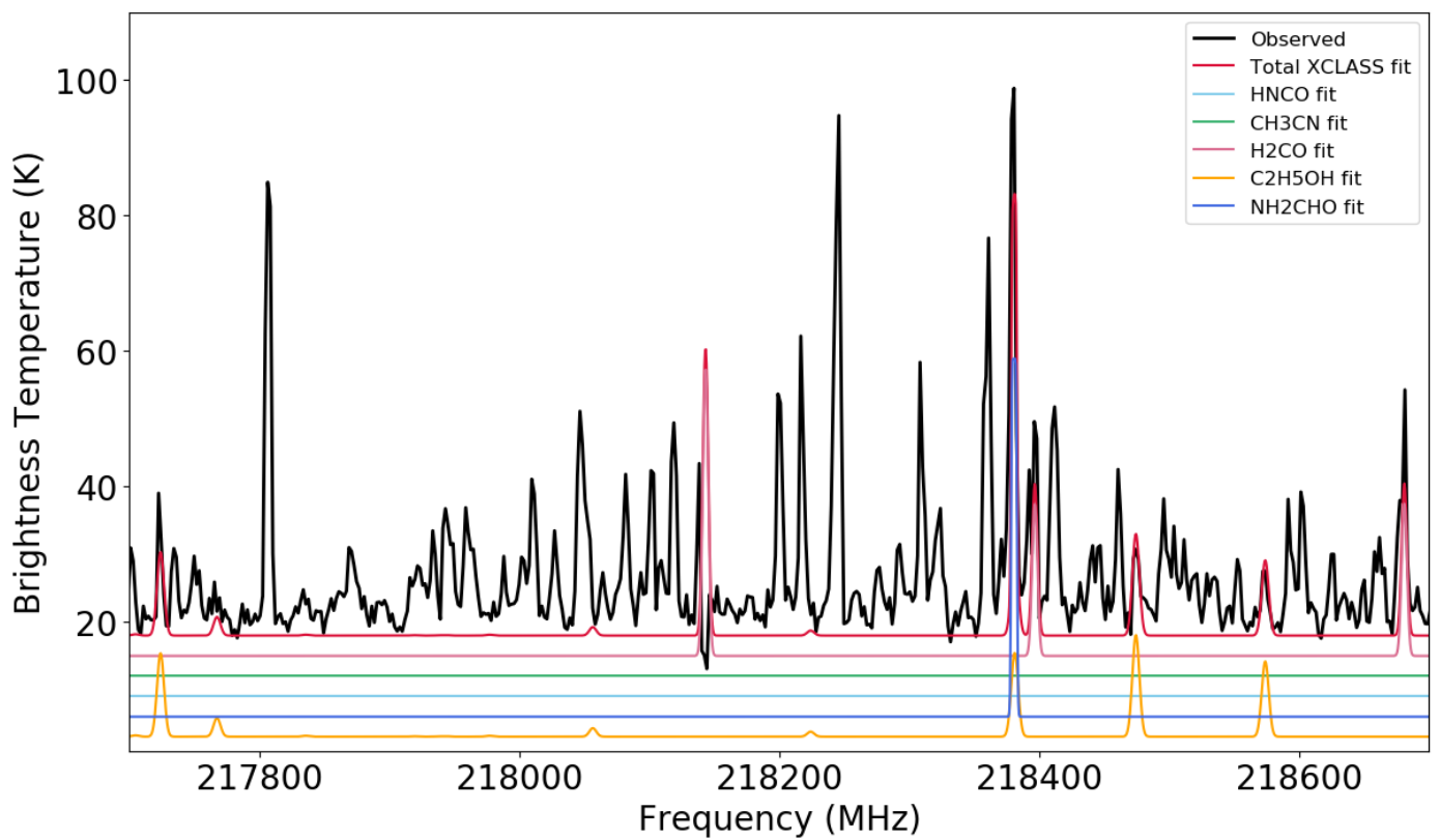
Fig. B.4. Spectral window from 217.7-218.7 GHz for G24 A1 containing NH 2 CHO (1) and H 2 CO (1), (2), and (3). NH 2 CHO (1) is blended with a transition of C 2 H 5 OH.
