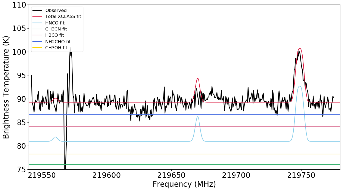
Fig. B.14. Spectral window from 219.5-219.8 GHz for G345 Main containing \text{HNCO} (3).
