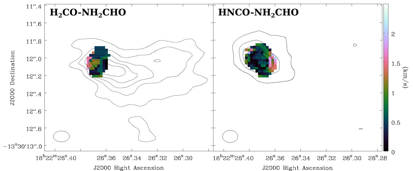
Fig. 8. Velocity difference (from first moment maps) at each pixel in G17 between (left) H 2 CO (2) and NH 2 CHO (1) and (right) HNCO (2) and NH 2 CHO (1). The contours show the integrated intensity maps for H 2 CO (2) and HNCO (2) as in Figure 4. The velocity scale is the same for both panels.
