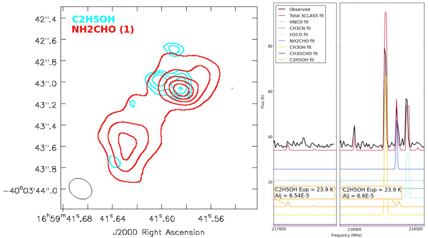
Fig. A.1. Right: Spectrum of G345 NW spur showing a \text{C}_2\text{H}_5\text{OH} transition ( 5_{3,3}-4_{2,2} ) at 217803 MHz with the same E_{\text{up}} and nearly equal A_{ij} as the \text{C}_2\text{H}_5\text{OH} transition ( 5_{3,2}-4_{2,3} ) that is blended with the \text{NH}_2\text{CHO} (1) transition (at 218461 MHz). Left: Contours of the integrated intensity map of this \text{C}_2\text{H}_5\text{OH} line is overlaid on the map of the \text{NH}_2\text{CHO} (1) transition to show that the strength and spatial extent is different.
