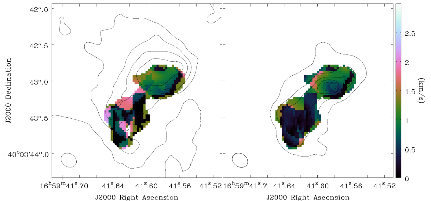
Fig. 14. Velocity dispersion difference (from second moment maps) at each pixel in G345 between (left) \text{H}_2\text{CO} (2) and \text{NH}_2\text{CHO} (1) and (right) \text{HNC} (2) and \text{NH}_2\text{CHO} (1). The contours show the integrated intensity maps for \text{H}_2\text{CO} (2) and \text{HNC} (2) as in Figure 6. The velocity scale is the same for both panels.
