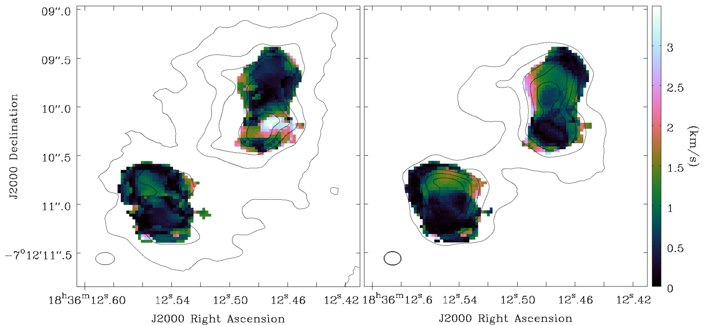
Fig. 13. Velocity dispersion difference (from second moment maps) at each pixel in G24 between (left) \text{H}_2\text{CO} (3) and \text{NH}_2\text{CHO} (2) and (right) \text{HNC} (1) and \text{NH}_2\text{CHO} (2). The contours show the integrated intensity maps for \text{H}_2\text{CO} (3) and \text{HNC} (1) as in Figure 5. The velocity scale is the same for both panels.
