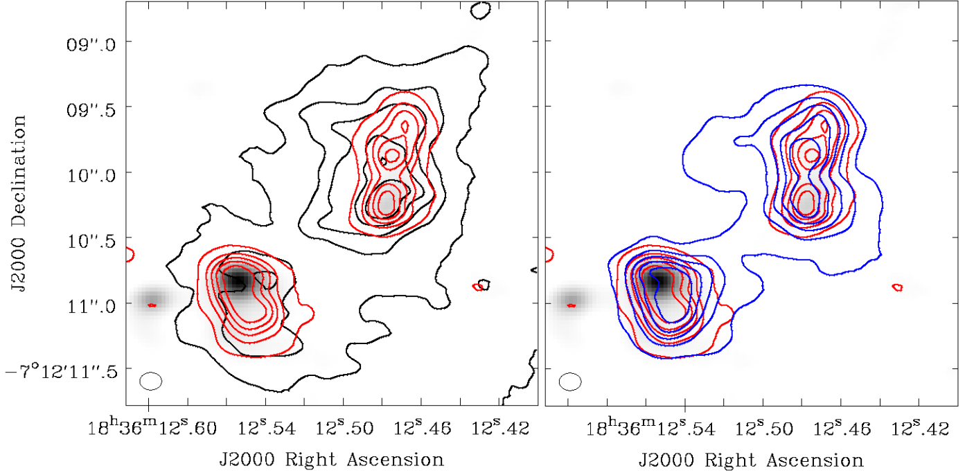
Fig. 5. G24 zeroth moment maps (contours) overlaid on the dust continuum (grayscale). Left: the black contours show the \text{H}_2\text{CO} (3) transition ( E_{\text{up}}=68.1 K) from 5\sigma to a peak of 0.674 Jy/beam \text{km s}^{-1} (contour levels 0.03, 0.16, 0.29, 0.42, and 0.55 Jy/beam \text{km s}^{-1} ). The red contours show \text{NH}_2\text{CHO} (2) emission ( E_{\text{up}}=78.9 K) from 5\sigma to 0.512 Jy/beam \text{km s}^{-1} (contour levels 0.026, 0.123, 0.220, 0.318, and 0.415 Jy/beam \text{km s}^{-1} ). Right: the blue contours show the extent of the \text{HNC} (1) emission ( E_{\text{up}}=58.0 K) from 5\sigma to 0.738 Jy/beam \text{km s}^{-1} (contour levels 0.031, 0.172, 0.314, 0.455, and 0.597 Jy/beam \text{km s}^{-1} ) with the red contours showing \text{NH}_2\text{CHO} (as in the left frame).
