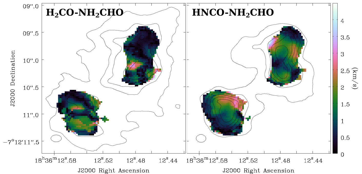
Fig. 9. Velocity difference (from first moment maps) at each pixel in G24 between (left) H 2 CO (3) and NH 2 CHO (2) and (right) HNCO (1) and NH 2 CHO (2). The contours show the integrated intensity maps for H 2 CO (3) and HNCO (1) as in Figure 5. The velocity scale is the same for both panels.
