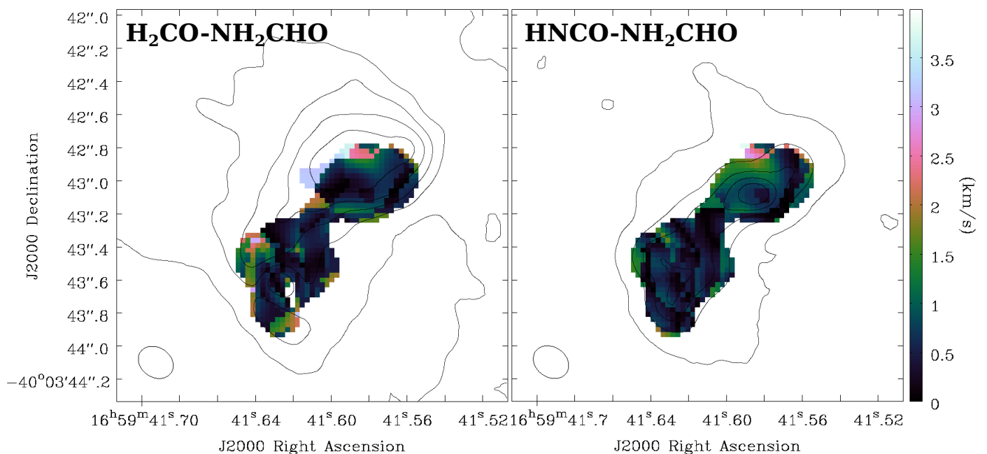
Fig. 10. Velocity difference (from first moment maps) at each pixel in G345 between (left) \text{H}_2\text{CO} (2) and \text{NH}_2\text{CHO} (1) and (right) \text{HNCO} (2) and \text{NH}_2\text{CHO} (1). The contours show the integrated intensity maps for \text{H}_2\text{CO} (2) and \text{HNCO} (2) as in Figure 6. The velocity scale is the same for both panels.
