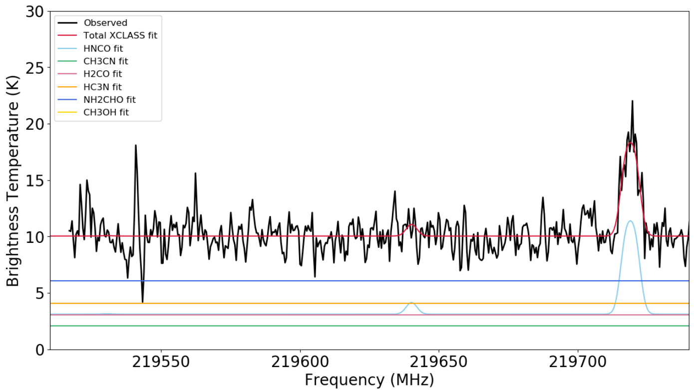
Fig. B.2. Spectral window from 219.5-219.8 GHz for G17 containing HNC(3).
