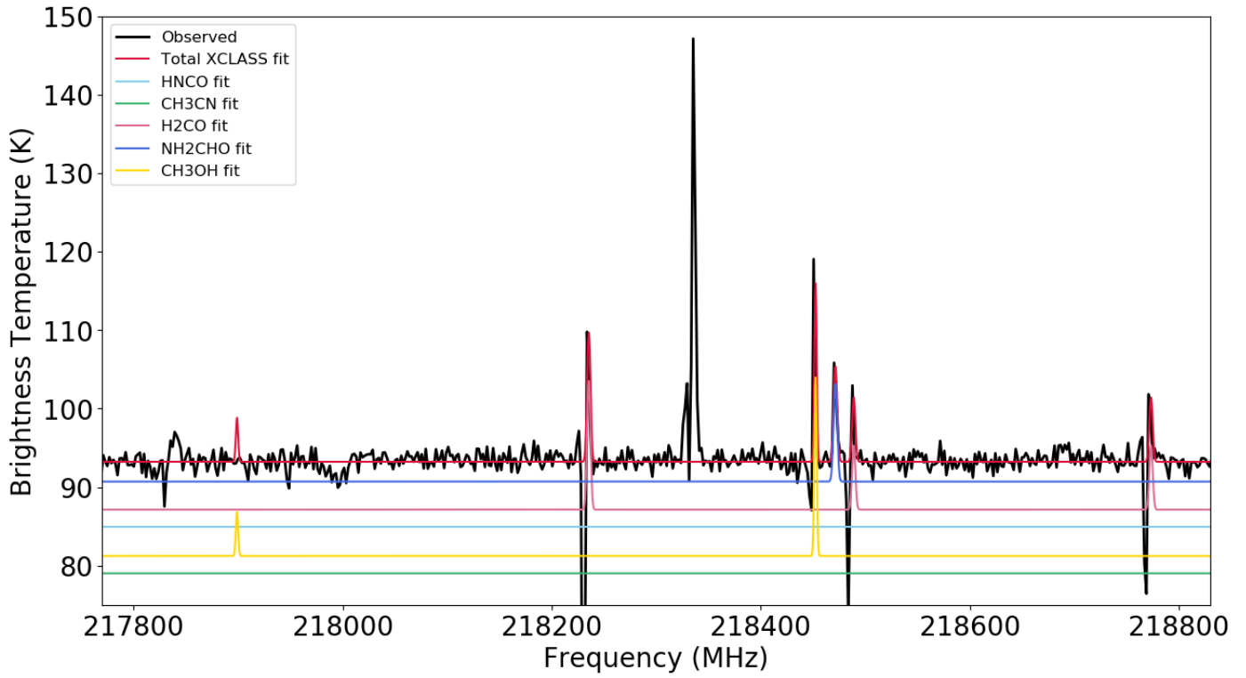
Fig. B.13. Spectral window from 217.8-218.8 GHz for G345 Main containing \text{NH}_2\text{CHO} (1) and \text{H}_2\text{CO} (1), (2), and (3).
