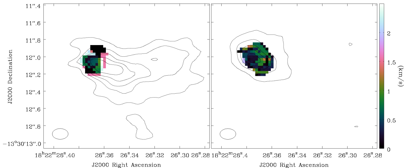
Fig. 12. Velocity dispersion difference (from second moment maps) at each pixel in G17 between (left) H 2 CO (2) and NH 2 CHO (1) and (right) HNCO (2) and NH 2 CHO (1). The contours show the integrated intensity maps for H 2 CO (2) and HNCO (2) as in Figure 4. The velocity scale is the same for both panels.
